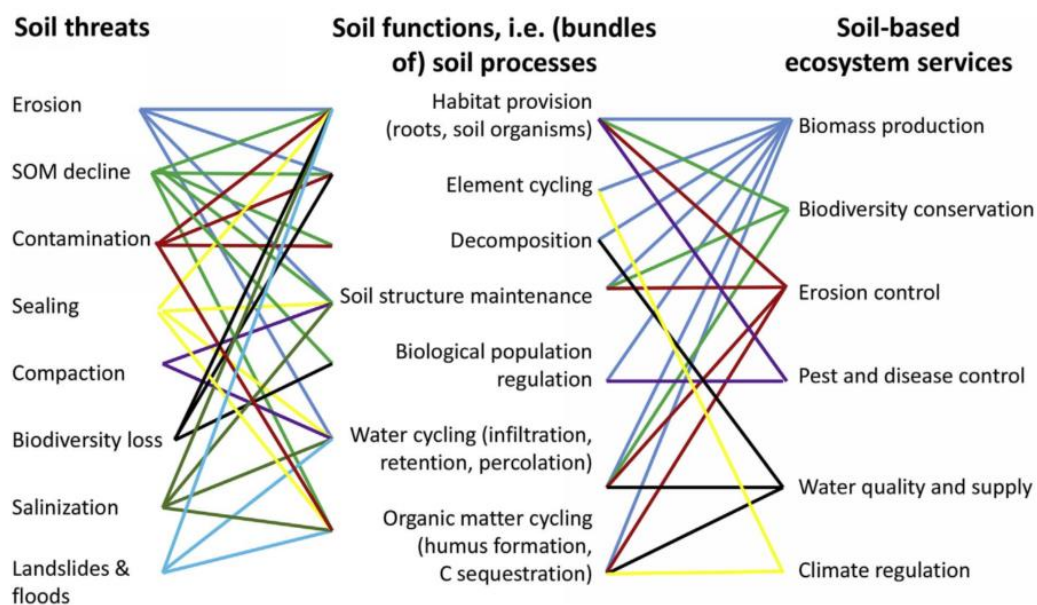
Figure 2-11. Linkages between soil threats, soil functions and soil-based ecosystem services. Further developed from the scheme presented by Kibblewhite et al. (Kibblewhite et al., 2008), from (Bünemann et al., 2018).
