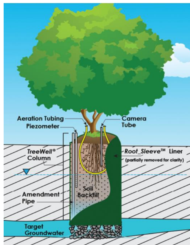
Figure 2-10. TreeWell phytoremediation system design, from TreeWell (geosyntec.com) .
