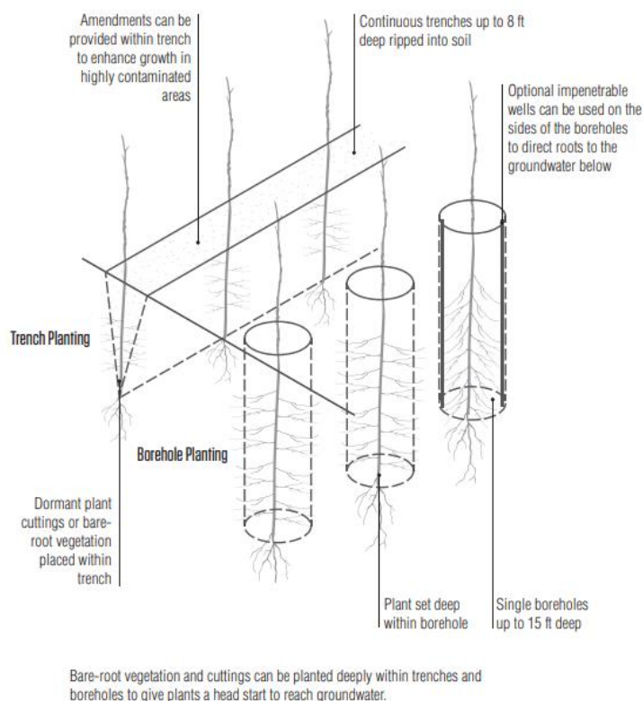
Figure 2-9. Deep-root planting techniques, from (Kennen and Kirkwood, 2015).
