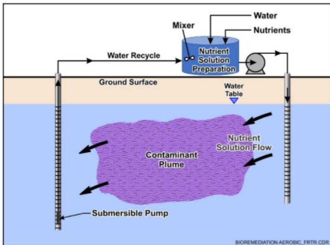
Figure 2-12. Conceptual diagram of enhanced aerobic biodegradation in groundwater, from Federal Remediation Technologies Roundtable (frtr.gov) .
