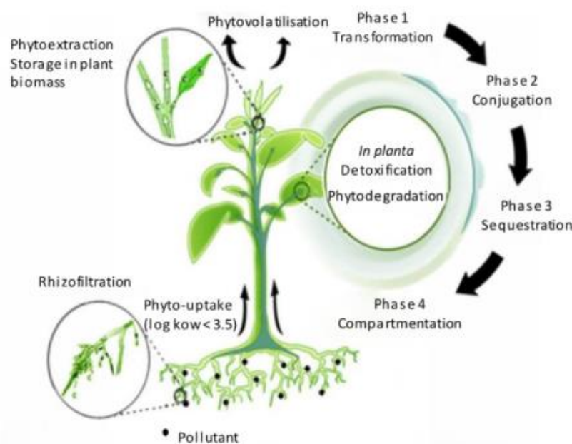
Figure 2-4. Green Liver model of plant response to xenobiotic compounds detailing plant uptake, transformation and degradation of contaminants in the plant, from (OVAM, 2019).
