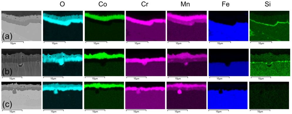
Figure 6.19: EDX maps of the cross-section of Ce/Co coated (a) 444 (b) 441 and (c) Crofer 22 APU exposed at 800 °C for 1000 h.
