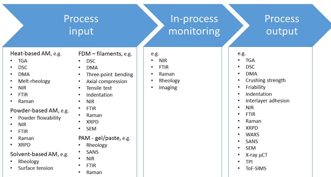
Fig. 8. Overview exemplifying the diversity of techniques used for characterization of feedstock or process input, in-process monitoring, and end-products or process output across AM of pharmaceutical oral products.
