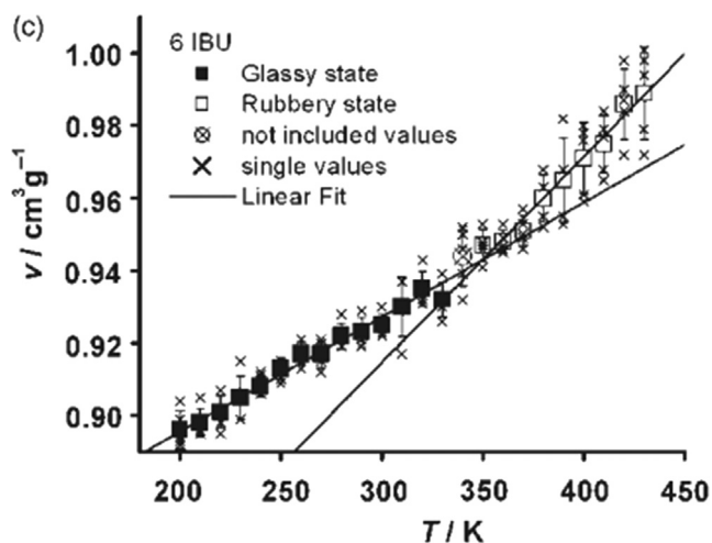
Fig. 7. Plot of the computed specific volume ( v ) versus temperature ( T ) for ibuprofen in Eudragit ® . The intersection between the two lines, resulting from a linear regression of the data points, corresponds to the glassy and rubbery states determined by the simulated T_g values. Figure reproduced with permission [253].
