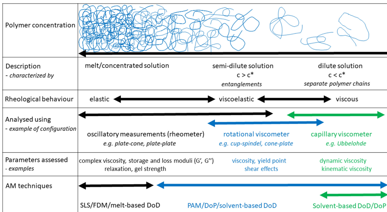
Fig. 6. Overview of polymer rheology, associated characterization techniques, and relevance in AM ( c = concentration, c^* = overlap concentration, G' = shear storage modulus, G'' = shear loss modulus).
