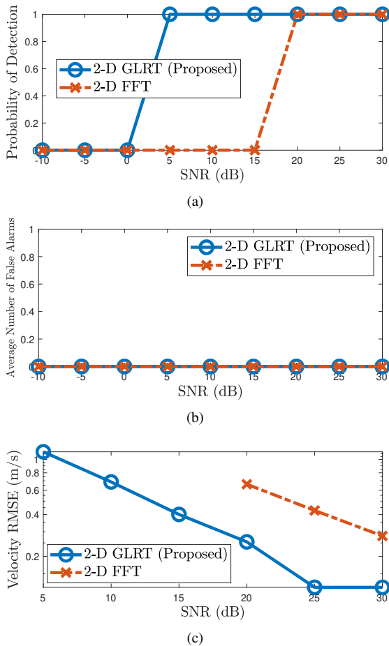
Fig. 7. Detection and estimation performance of the considered OTFS radar algorithms with respect to SNR in the ICI-dominant regime. (a) Probability of detection, (b) average number of false alarms, and (c) velocity RMSE.
