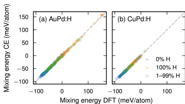
Figure 2. Comparison of mixing energies as calculated by DFT and as predicted by CEs for all structures in the training set for AuPd:H (a) and CuPd:H (b). The structures are colored according to their H coverage. The CE predictions agree well with the DFT calculations regardless of H coverage.
