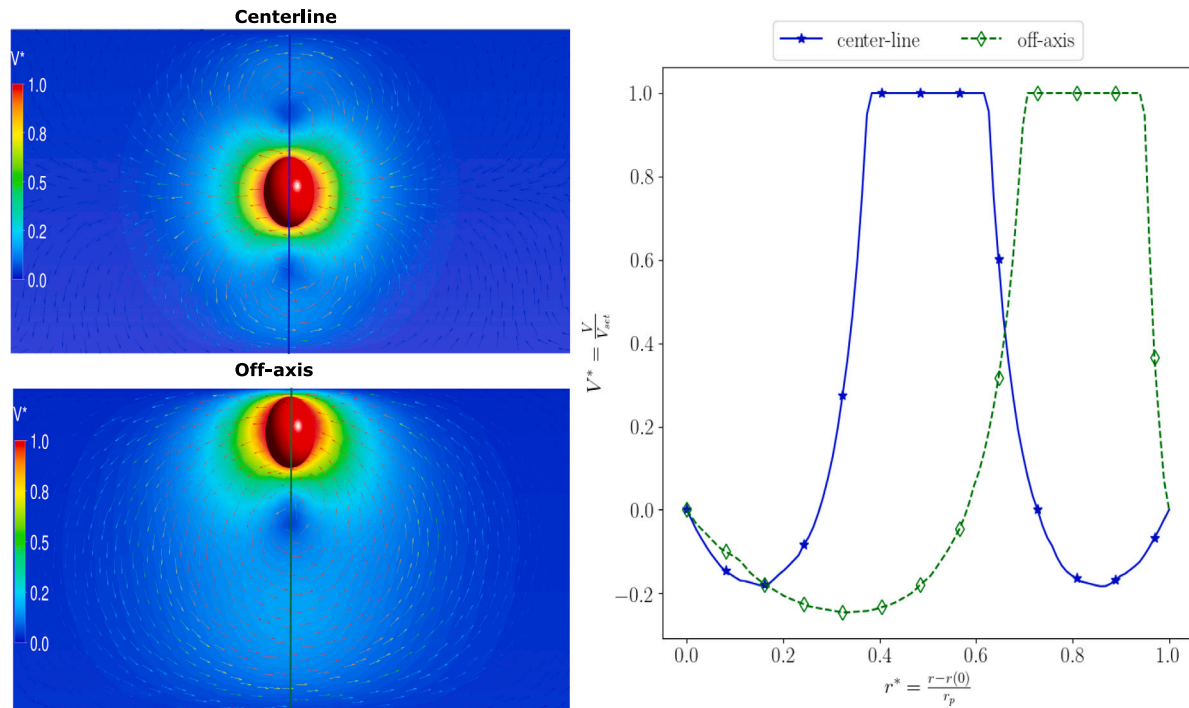
Fig. 5. Left panel: Re-circulation zones around a particle located at centerline and off-center positions. Contours of normalized co-axial fluid velocity ( V^* = \frac{V_z}{V_s} ) overlaid with flow vectors along the same direction (from the steady-state CFD simulations) in an x - z plane at 6.5d_p < x < 13.5d_p (i.e. a 6 d_p co-axial span around the particle), y = w/2 and 0 < z < a . This normalization is done for a simplified visualization of the hydrodynamic zones. Right panel: V^* over a line passing through the center of the particle (i.e. x = l/2 , y = w/2 and 0 < z < a ) plotted as a function of the non-dimensional distance r^* = \frac{r-r(0)}{r_p} ( r^* = 0 and r^* = 1 represent the location of the walls along the z -direction) at B = 4.6 . Note the lack of a flow reversal in the region between the particle and the wall in the off-axis configuration.
