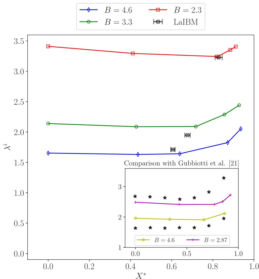
Fig. 4. Directional reduction in mobility, \lambda^i , along the co-axial direction at the blockage ratios ( B ) 4.6, 3.3 and 2.3, respectively, for the CFD simulations in a square micro-channel. Here, X^* is the non-dimensional z-location of the particle between the center of the channel and the walls. The inset shows the comparison between the DPD data of Gubbiotti et al. (2019) and our steady state CFD results in a cylindrical channel. Also plotted are the mean \lambda^i , extracted from the particle mean-squared behavior in the LaIBM framework with an error bar indicating the span of X^* visited by the particle in the simulation. Note the minimum in \lambda^i as the particle is shifted off-axis.
