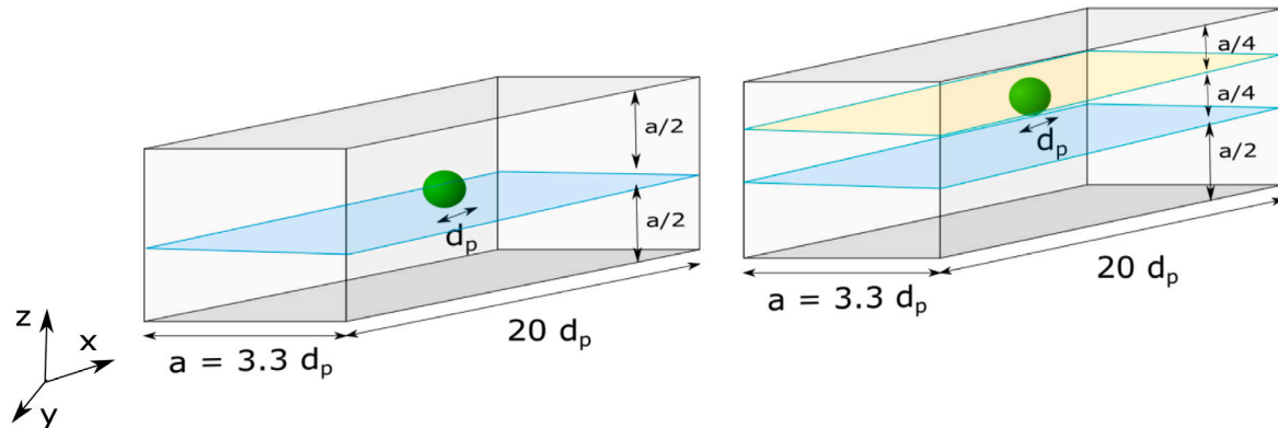
Fig. 2. Examples of the simulation domain: diffusion in the vicinity of the centerline (at a/2 ) inside a straight square micro-channel (left panel) and diffusion originating from an off-axis position (at a/4 ) inside a straight square micro-channel (right panel). The dimensions are in terms of the particle diameter ( d_p ). Note that x is the co-axial direction, while z is the wall-normal direction under study here. The corresponding x - y planes at different z positions are depicted in the square micro-channel schematics.
