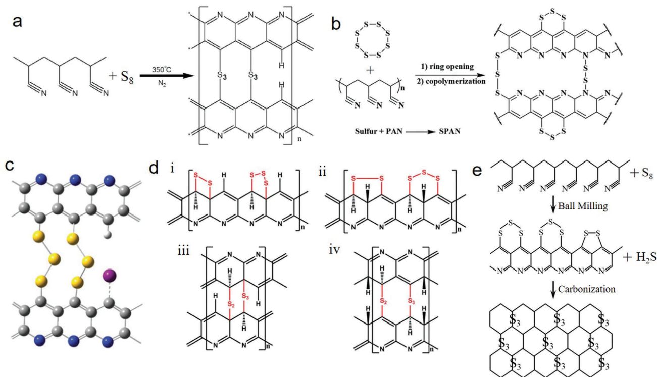
Figure 4. Schematic of covalent structure of some SPAN materials with -\text{[S]}_n \leq 3- chains. a) Reproduced with permission. [58] Copyright 2020, Royal Society of Chemistry. b) Reproduced with permission. [77] Copyright 2010, MDPI. c) Reproduced with permission. [74] Copyright 2019, Elsevier. d) Reproduced with permission. [44] e) Reproduced with permission. [33] Copyright 2015, American Chemical Society.
