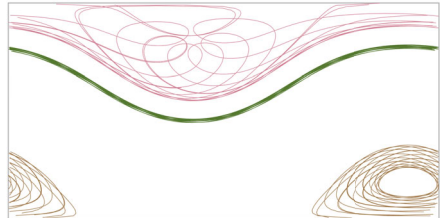
(b) 3 point-vortices, non-vanishing momentum. Solutions are integrable.
