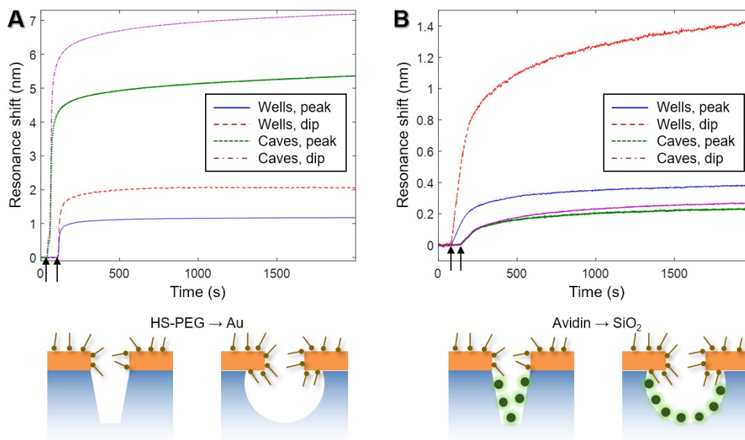
Figure 18. Real-time plasmonic response from location-specific molecular binding to the nanostructures; (A) Thiolated 2 kDa poly(ethyleneglycol) binding to Au; (B) Protein adsorption to the silica cavities. The temporal resolution is 250 ms and the data is not smoothened. The nanowells were 120 nm deep and 100 nm in diameter. The nanocaves were 70 nm in diameter and 100 nm deep. (Figure and caption from Paper I ).
