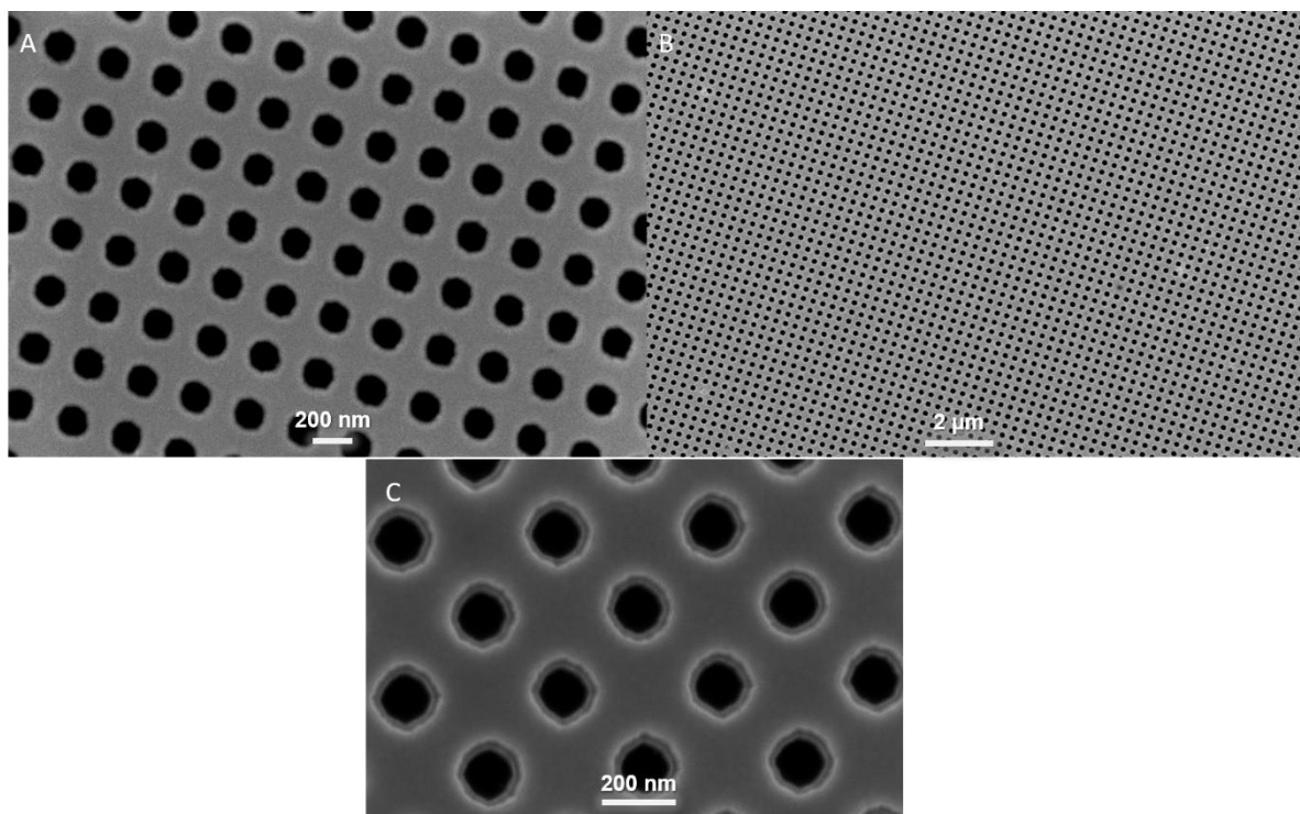
Figure 13. SEM images of membrane nanopores after lift-off (A) , (B) After RIE (C) After ion beam milling.
