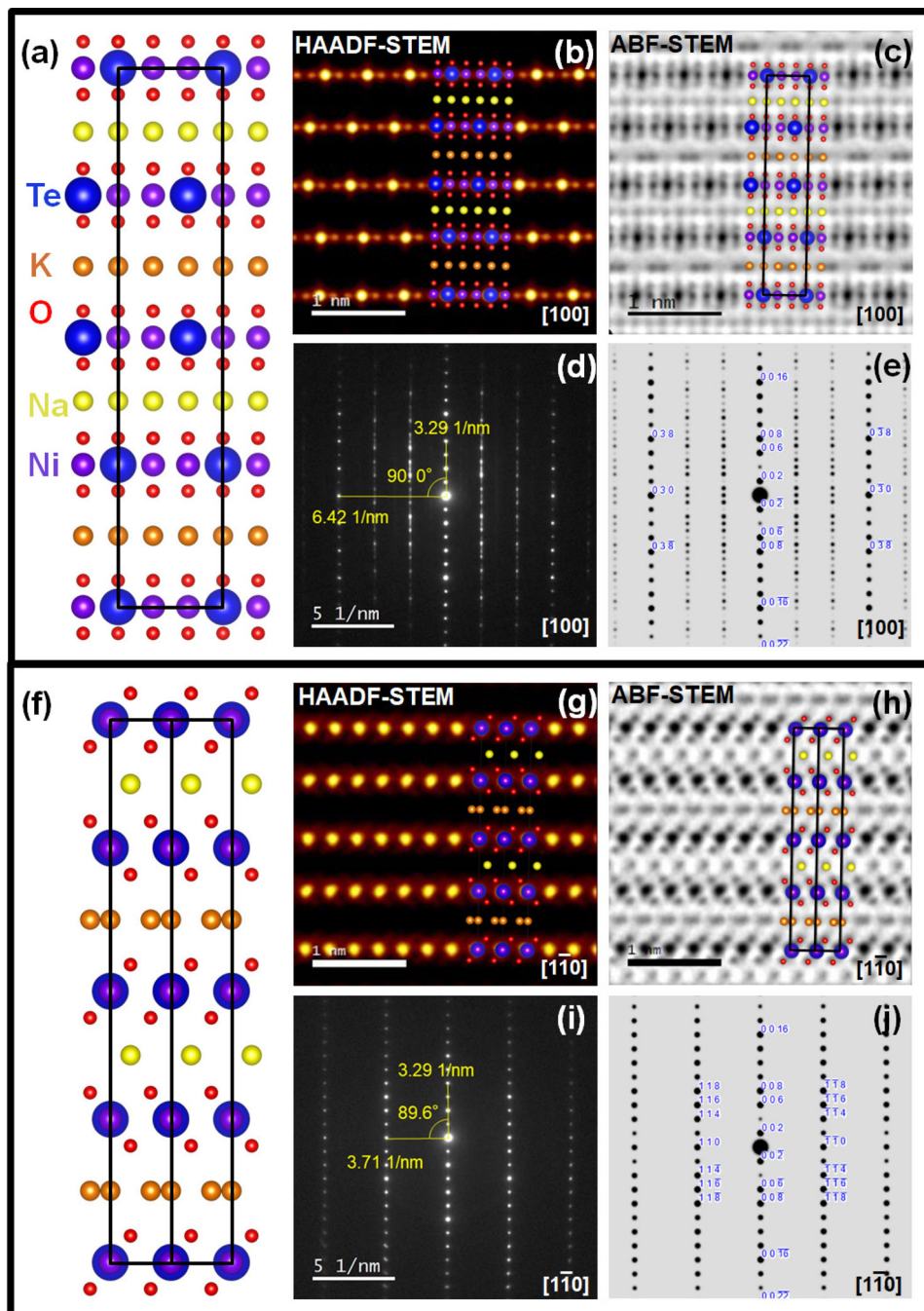
Fig. 3 Aperiodic atomic structure of \text{NaKNi}_2\text{TeO}_6 along the [100] and the [\bar{1}\bar{1}0] zone axes. a Atomistic model of the average aperiodic structure of \text{NaKNi}_2\text{TeO}_6 acquired based on STEM analyses along the [100] zone axis. Black lines show the partial unit cell. b Superimposition of the model on a HAADF-STEM image, showing an excellent overlap between the positions of the Ni and Te atoms in the model that is in accord with the intensity distribution of the atom spots observed in the image. c Superimposition of the model on an annular bright-field (ABF) image, affirming the atomic positions of Na, K and O. d Selected area electron diffraction (SAED) patterns taken along the [100] zone axis revealing spot shifts and streaks that are suggestive of the existence of aperiodicity. e Corresponding kinematic simulations based on the structural model shown in (a) , showing agreement with the experimental results in (d) . f Atomistic model of \text{NaKNi}_2\text{TeO}_6 acquired based on STEM analyses along the [\bar{1}\bar{1}0] zone axis. Black lines show the partial unit cell. Note the difference in the arrangement of atoms between Na (yellow) and K (orange) crystallographic sites. g Superimposition of the model on a HAADF-STEM image, affirming the atomic positions of Ni and Te. h Superimposition of the model on an ABF-STEM image, also showing an excellent overlap between the positions of the Na, K and O atoms in the model that is in accord with the intensity distribution of the atom spots observed in the image. i SAED patterns taken along the [\bar{1}\bar{1}0] zone axis and j the corresponding kinematic simulations, validating good agreement with the experimental results shown in (d) .
