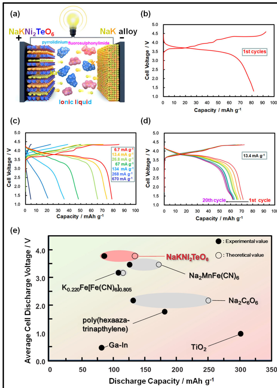
Fig. 6 Electrochemical energy storage performances of NaKNi 2 TeO 6 as a cathode active material for NaK cells. a A schematic illustration of a dual (Na and K-ion) battery using NaKNi 2 TeO 6 as cathode and dendrite-free NaK liquid alloy as anode. b Voltage-capacity profiles of NaKNi 2 TeO 6 dual-cation cathode material in a cell using NaK as anode during initial cycling at a specific current of 6.7 mA g -1 . The voltage range was set at 4.6–1.3 V. The electrolyte used was a pyrrolidinium-based dual-metal-cation ionic liquid, comprising equimolar amounts of Na and K (i.e., Na 0.10 K 0.10 Pyr 0.80 FSI). Details regarding the cell assembly are provided in the “Methods” section. c Voltage-capacity profiles at various specific currents under a voltage range of 4.35–1.3 V. d Cyclability performance at a specific current of 13.4 mA g -1 rate upon subsequent cycling (20 cycles). e Voltage-capacity plots of cathode materials reported so far for NaK batteries. Comparison data of NaKNi 2 TeO 6 with reported cathode materials for NaK batteries are furnished as Supplementary Table 7. For clarity, the methodology to calculate the average discharge voltage is reported in the Supplementary Information section (Supplementary Fig. 26).
