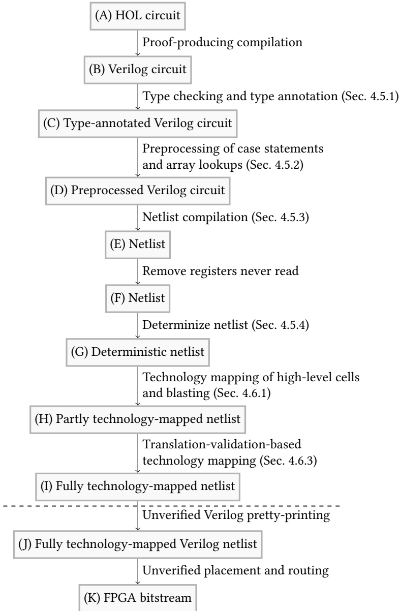
Figure 4.1. An overview of Lutsig’s compilation passes and illustration of how Lutsig fits into circuit development.
