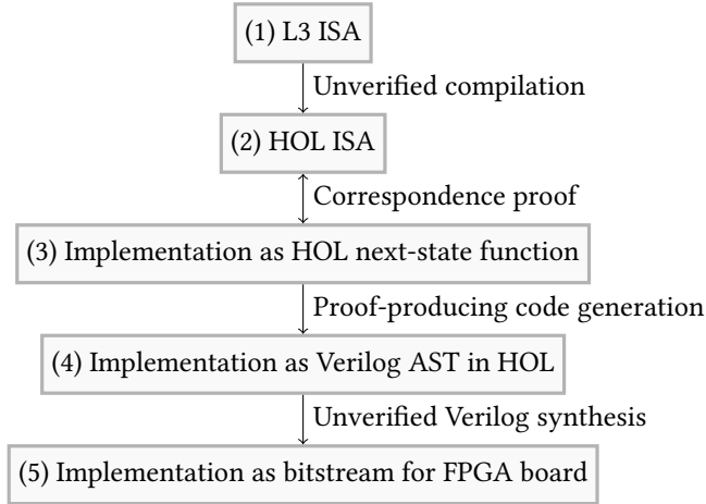
Figure 2.1. The layers involved in the construction and verification of the Silver processor.
