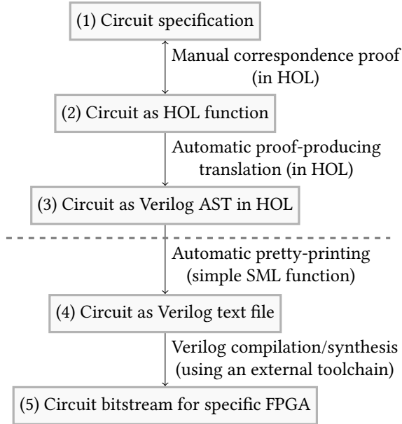
Figure 3.1. An overview of our hardware-development methodology. For non-trivial circuits, human-guided proofs are needed for the connection between layers 1 and 2, whereas the other steps are always automatic. The correspondences above the dotted line are proved functionally correct, and the correspondences below the dotted line are not covered by our formal development. The main focus of this paper is the translator connecting layers 2 and 3.
