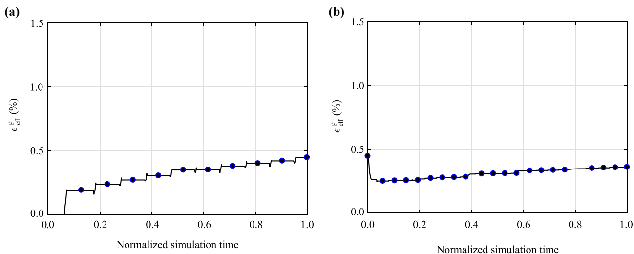
Fig. 12 Viscoplasticity model when biaxial parameter is set to \beta_i = 1 . Case S160, 1 band 50 mm. Evolution of the equivalent von Mises plastic strain \epsilon_{\text{eff}}^{\text{P}} at 1.4 mm below the center of wheel–railwheel contact a during the first 10 rolling passages at room temperature and b during the braking cycle. Solid circles indicate the beginning instance of every rolling passage
