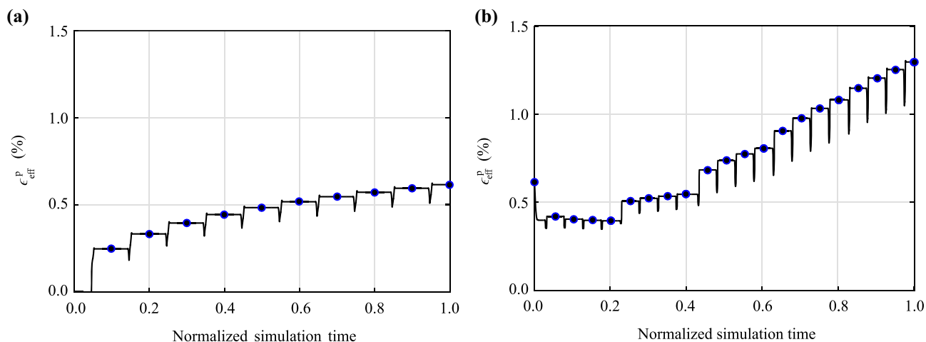
Fig. 11 Plasticity model. Case S160, 1 band 50 mm. Evolution of the equivalent von Mises plastic strain \epsilon_{\text{eff}}^{\text{P}} at 1.4 mm below the center of wheel–railwheel contact a during the first 10 rolling passages at room temperature and b during the braking cycle. Solid circles indicate the beginning instance of every rolling passage
