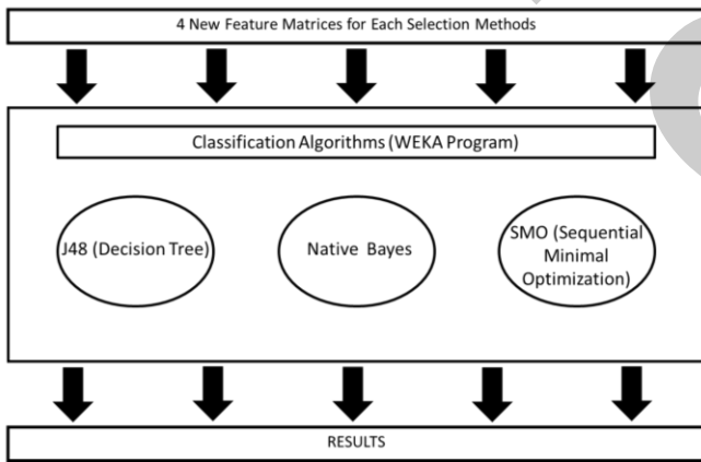
Fig. 2. Classification Algorithms
