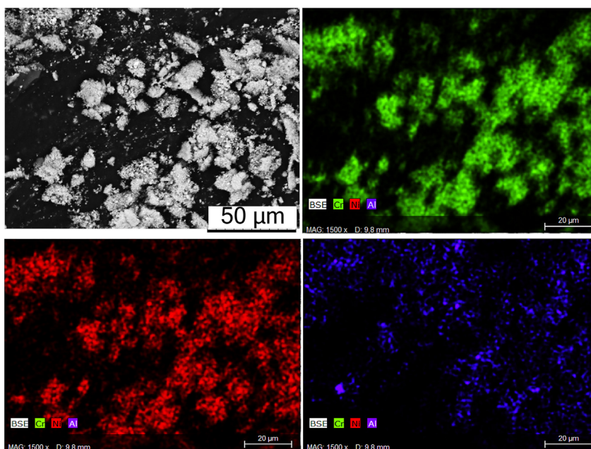
Fig. 13 – SEM/EDS analysis of the wear debris obtained from the \text{Cr}_3\text{C}_2\text{-NiCr} reference coating.
