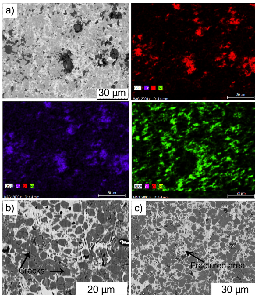
Fig. 12 – Top surface SEM micrographs (BSE mode) of worn \text{Cr}_3\text{C}_2\text{-NiCr} reference coating showing a) tribo-oxidation and its corresponding EDS analysis b) Abrasive grooving c) brittle fracture.
