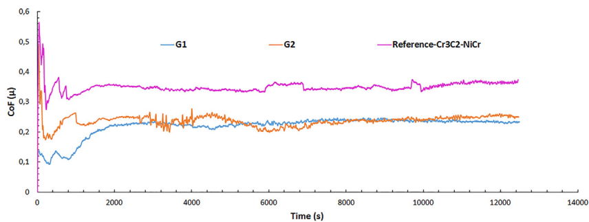
Fig. 10 – CoF comparison of the Cr 3 C 2 -NiCr reference coating, G1 coating and G2 coating.
