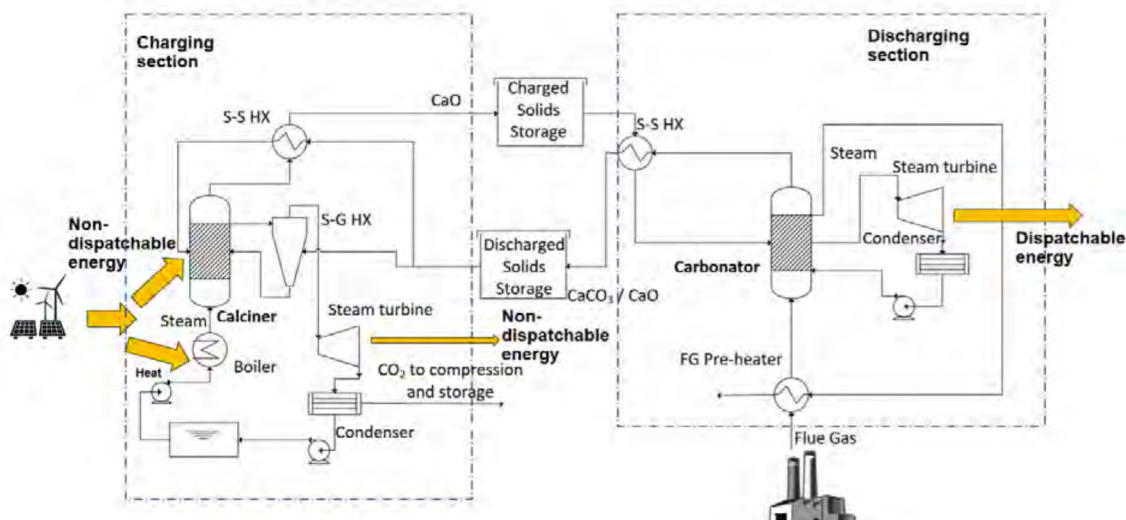
Figure 1. Schematic diagram of the investigated process. Note that the non-dispatchable energy input is in the form of high-temperature heat and the produced energy is in the form of electricity.
