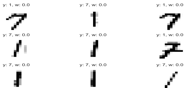
Figure 4: Example of images that where mislabeled and that DRFit could detect. Above each example is the label the model was given and the weight that DRFit assigned to the data point.
