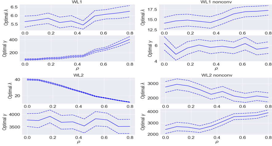
Figure 6: The average optimal parameters for EWL and EWR for correlated covariates as functions of \rho . The dashed lines correspond to the estimated 95% confidence intervals based on the 100 sampled points.
