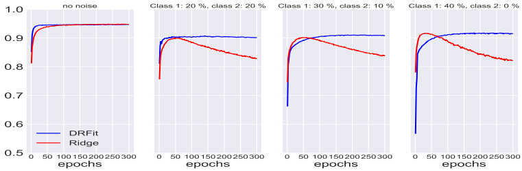
Figure 6: The average accuracy on a test data for DRFit and pure ridge regularization during training when trained on the classes cars and planes in the cifar10 dataset. In order to vary the noise we have done this in four different label noise settings. One with equally amount of noise in both classes, one with 30% noise in class one and 10% in class two, one with 40% noise in class one and no noise in class two and one setting with no label noise in the training data. In order to get a better comparison the runs that crashed are removed.
