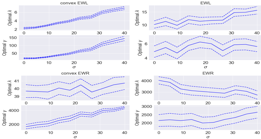
Figure 5: The average optimal hyper-parameters with respect to MSE for EWL and EWR, both in the convex and in the non-convex setting with uncorrelated covariates as functions of \sigma . The dashed lines correspond to the estimated 95% confidence intervals based on 100 sample points.
