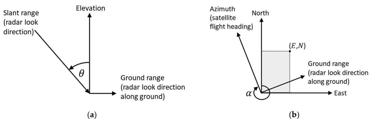
Figure 2. Acquisition geometry for a right-looking SAR system, with the incidence angle ( \theta ) and heading angle ( \alpha ) shown together with the principal axes of a SAR acquisition. (E, N) are the respective east and north coordinates of a grid cell. (a) Elevation plane; (b) ground plane.
