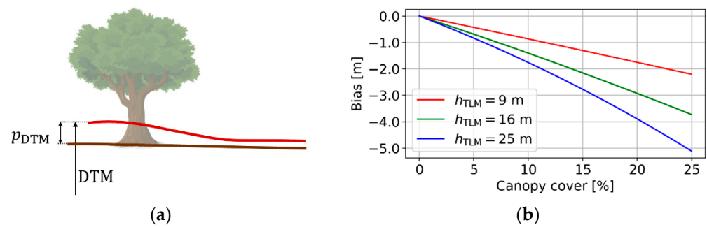
Figure 4. The effect of vegetation bias from the DTM on tree height estimation. (a) Vegetation bias is the offset between the DTM and the true ground surface, caused by vegetation objects. (b) Sample results showing the effect of vegetation bias from the DTM on tree height estimation, as modelled by TLM for \kappa = 0.063 (HOA \approx 100 m).
