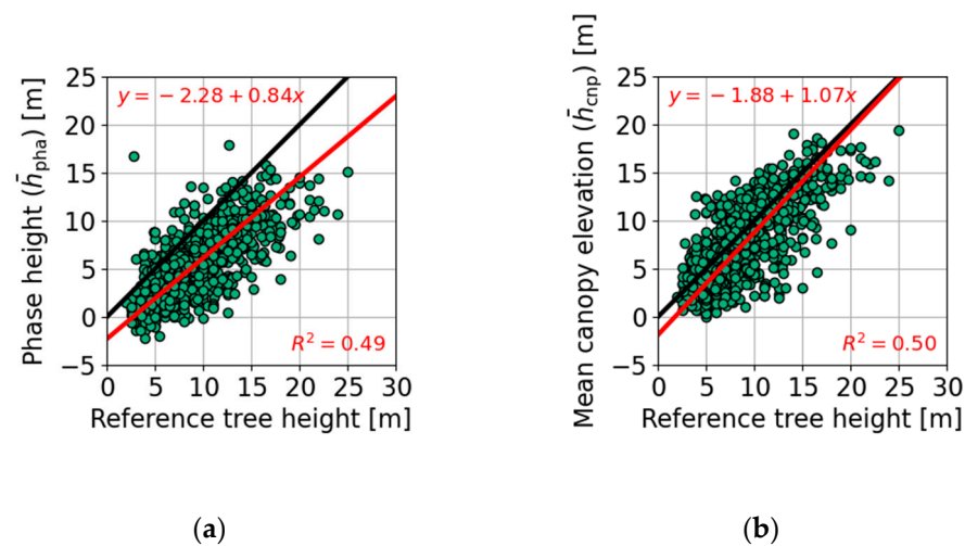
Figure 7. Comparison of the estimated (a) phase height ( \bar{h}_{\text{pha}} ) and (b) mean canopy elevation ( \bar{h}_{\text{cnp}} ) with reference in situ tree height ( h_{\text{top}} ) for all 915 trees from 15 species/genera inventoried during three field campaigns in Saponé. Green dots indicate individual trees. The solid red line describes the bias in the data, and it was obtained by fitting a linear model to the data using orthogonal distance regression. The solid black line shows the zero-bias case. The corresponding estimation statistics are shown in Table 5.
