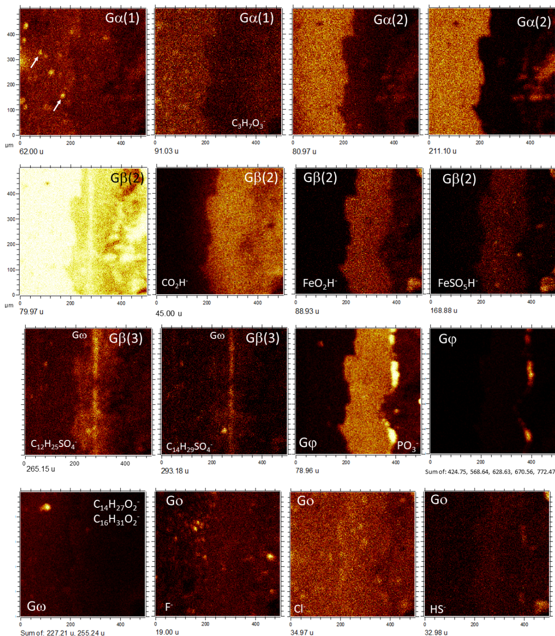
Figure 7. Identification of the morphological groups through the anion ToF-SIMS images in TA2. As for cations, it has been characterized Gα, Gβ, Gγ, and Gφ, plus a new group Gω that includes the distribution of different anions with unrelated patterns. Minor pattern changes inside Gα and Gβ have suggested to separate them into several subgroups as it has also observed for the TA2 cation groups. The HS - distribution classified into Gω follows the phosphatic discontinuous laminae and the NH 4 + -bearing nodules, which are associated with the presence of amino acids. The ToF-SIMS images were obtained from a rasterized surface area of a 500 μm square.
