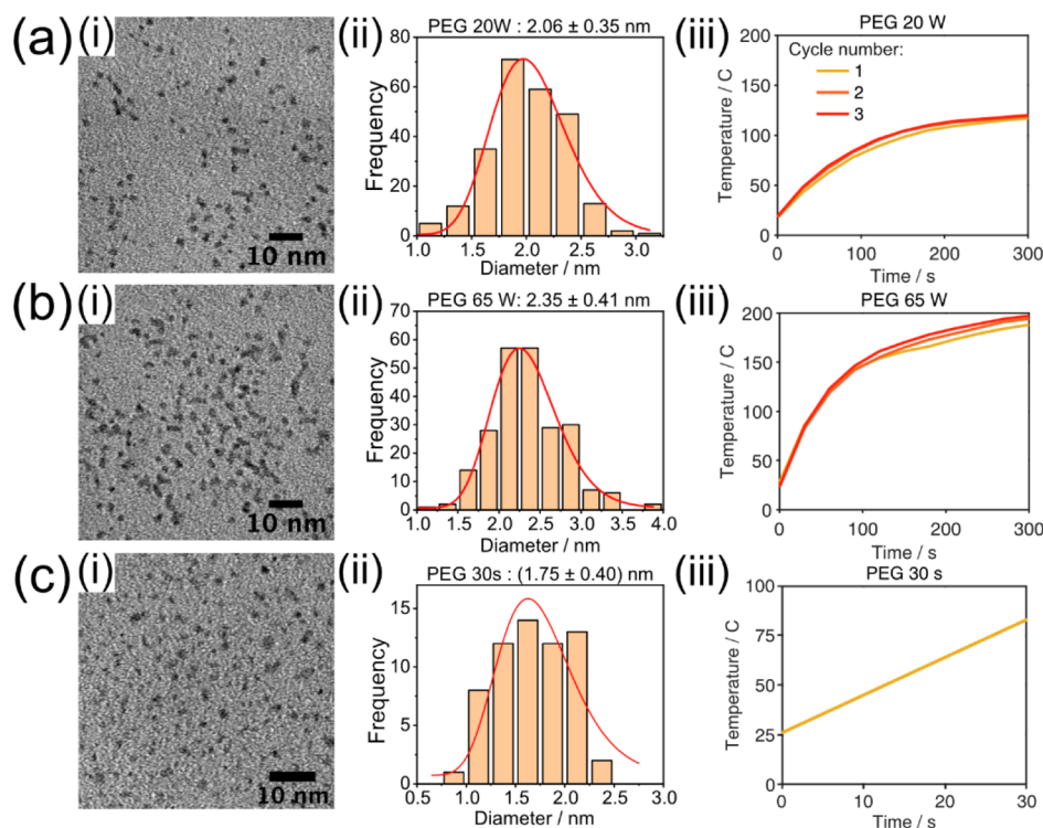
Figure 4. Effect of sputtering power and time on Pt nanoparticle size in PEG. (a) 20 W for 3 × 300 s, (b) 65 W for 3 × 300 s, and (c) just 30 s of sputtering at 50 W. (i) Corresponding TEM images, (ii) nanoparticle size distribution, and (iii) temperature development of the substrate liquid throughout the sputtering cycles.
