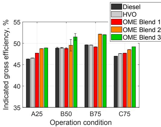
Fig. 1. Heavy duty engine: indicated thermal efficiency.
