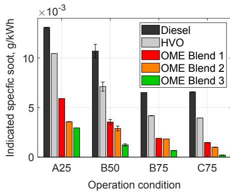
Fig. 5. Heavy duty engine: Indicated specific soot emissions.
