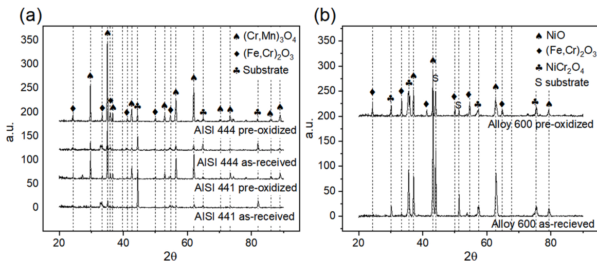
Fig. 6. (a) XRD analysis of AISI 441 and AISI 444 in as-received and pre-oxidized conditions exposed at 650 °C for 500 h. (b) XRD analysis of alloy 600 in as-received and pre-oxidized conditions exposed at 650 °C in air + 3 % H 2 O for 500 h.
