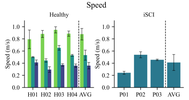
Fig. 3. Walking speeds for healthy and iSCI subjects. Healthy subjects performed the walking trials at 3 speeds (normal, slow and very slow) whereas iSCI subjects performed only single speed walking. All walking speeds were self-paced.
