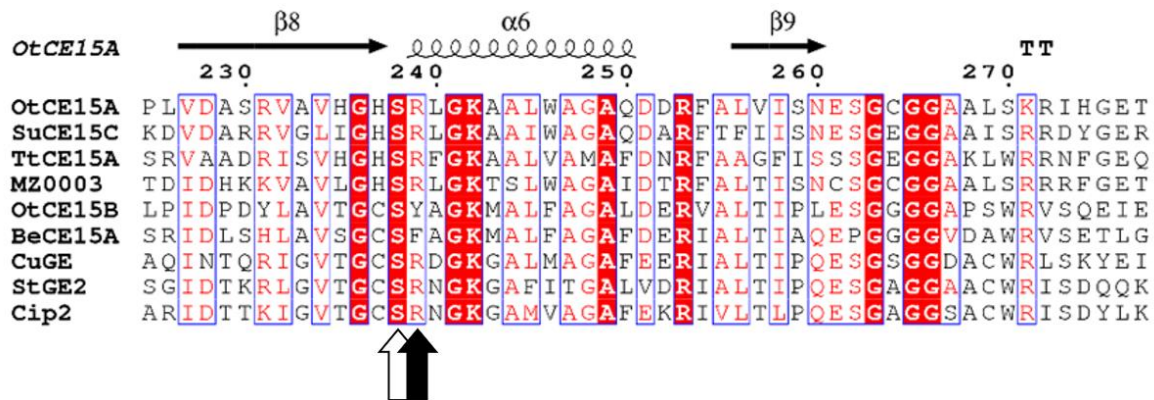
Figure 9: Sequence-based alignment of BeCE15A showing the region of the catalytic serine and the neighboring phenylalanine residue. The figure was adapted from paper III. The secondary structural elements of OtCE15A (101), a glucuronoyl esterase from Opitutus terrae with published structure (PDB accession 6SYU) served as template. The catalytic serine is marked with a white arrow, the usually conserved arginine residue that is substituted in BeCE15A with phenylalanine and in OtCE15B with tyrosine is marked by a black arrow.
