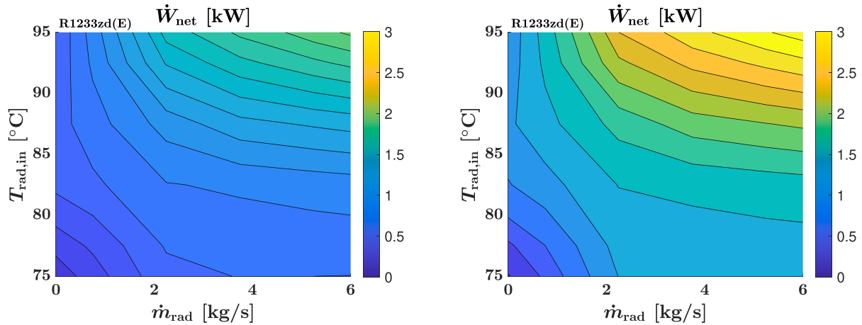
Fig. 24. Net shaft power for the standard (left) and optimum (right) system as functions of the radiator mass flow and inlet temperature. The values at the edges were linearly extrapolated.
