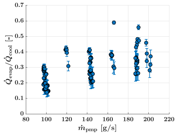
Fig. 7. Absolute (left) and relative (right) evaporator heat transfer rate as a function of the mass flow.
