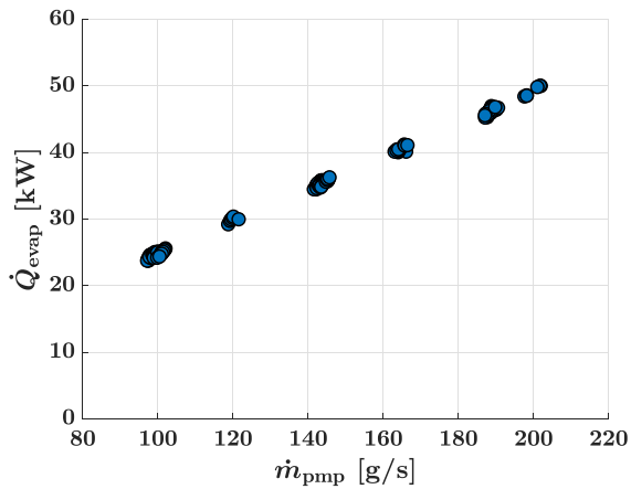
Fig. 7. Absolute (left) and relative (right) evaporator heat transfer rate as a function of the mass flow.
