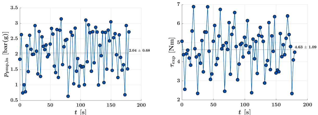
Fig. 27. Fluctuations in the pump inlet pressure (left) and the expander torque (right).
