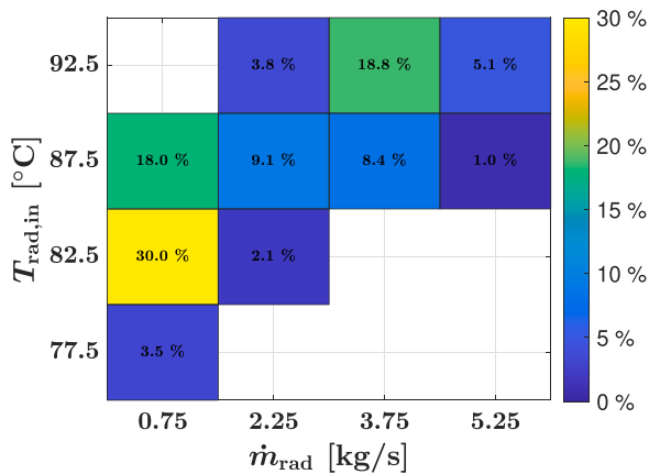
Fig. 23. Relative time distributions of the different inlet conditions (radiator mass flows and inlet temperatures) for the driving cycle. The total drive cycle time ( \Delta t_{dc} ) is 3832 s.
