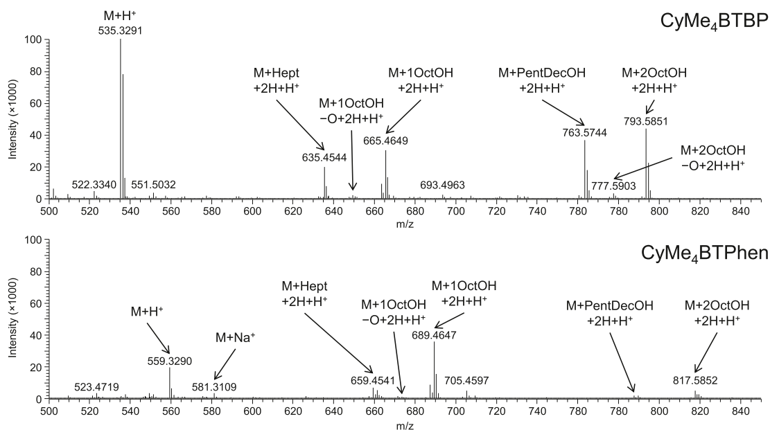
Fig. 3. Mass spectra of 10 mmol L -1 CyMe 4 BTBP (top) and CyMe 4 BTPPhen (bottom) in 1-octanol irradiated to 132 kGy absorbed dose without contact to nitric acid. M = CyMe 4 BTBP or CyMe 4 BTPPhen, OctOH = \alpha -hydroxyoctyl, PentDecOH = 8-hydroxypentadecanyl, Hept = heptyl.
