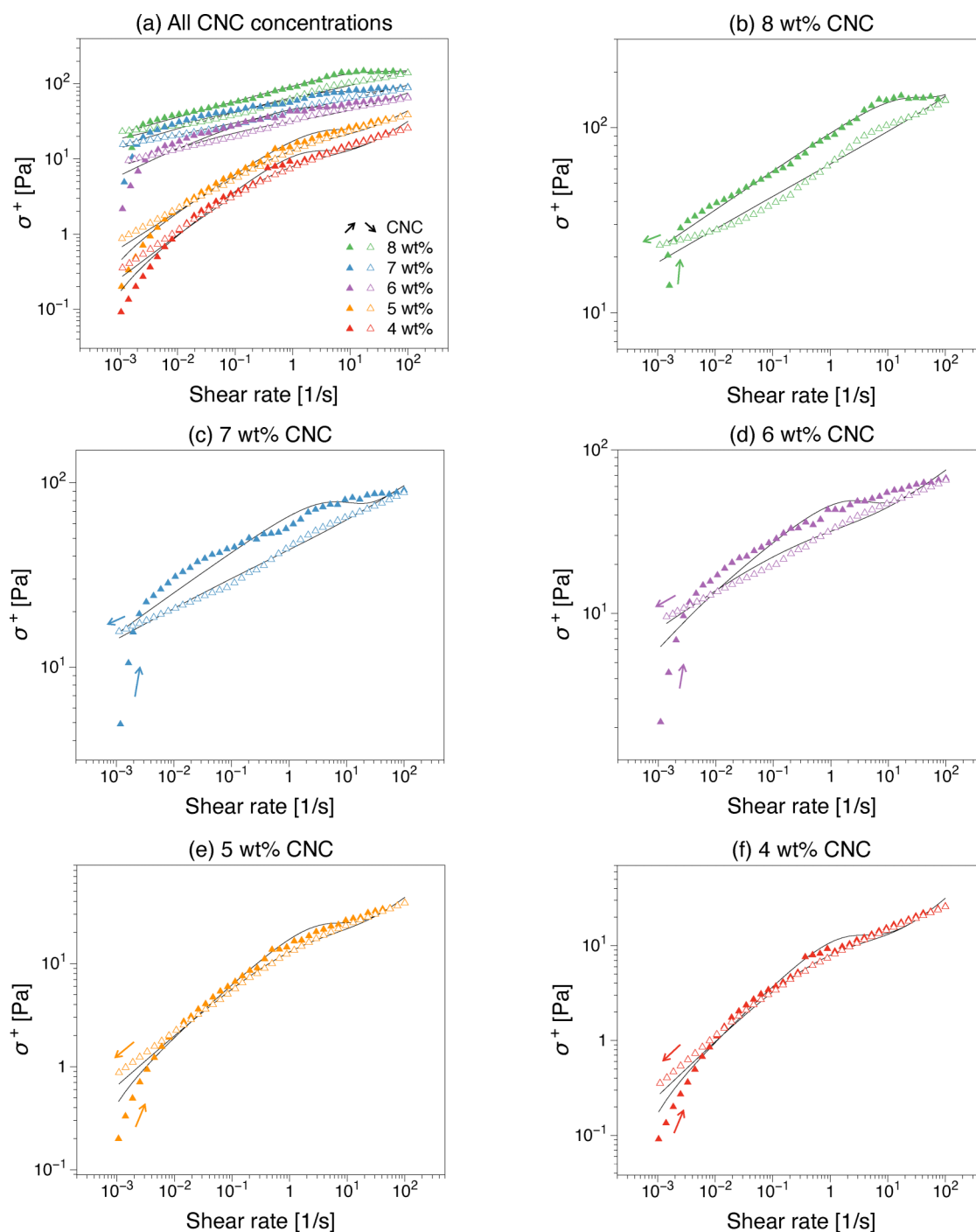
FIG. 8. Flow curves, shear stress vs shear rate, obtained by increasing \dot{\gamma} from 0.001 to 100\text{ s}^{-1} and then decreasing \dot{\gamma} over the same range with a waiting time of 10\text{ s} per data point: (a) comparison between all CNC concentrations; (b) 8, (c) 7, (d) 6, (e) 5, and (f) 4 wt. % CNC suspensions. The continuous line represents the numerical modeling of the thixotropic behavior according to Eqs. (1) and (2).
