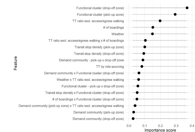
Fig. 7. Feature/feature interaction score indicating importance in predicting whether a ride-sourcing trip is transit-competing.
