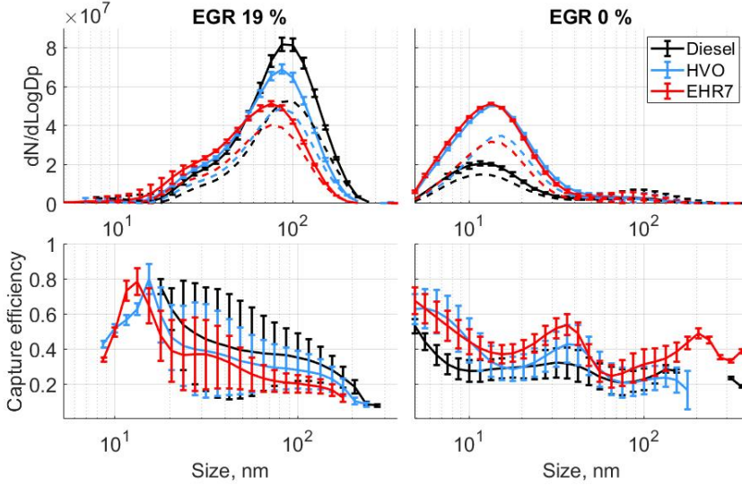
Figure 4.10.: PSD and capture efficiency for the double pre/main/post injection strategy with 19 % EGR (left) and 0 % EGR (right). In the upper images, continuous lines indicate results obtained without the thermodenuder while dashed lines represent those obtained with the thermodenuder. Standard deviations are not shown for the PSD after passage through the thermodenuder for clarity. However, the errors were approximately equal for both measurements.
