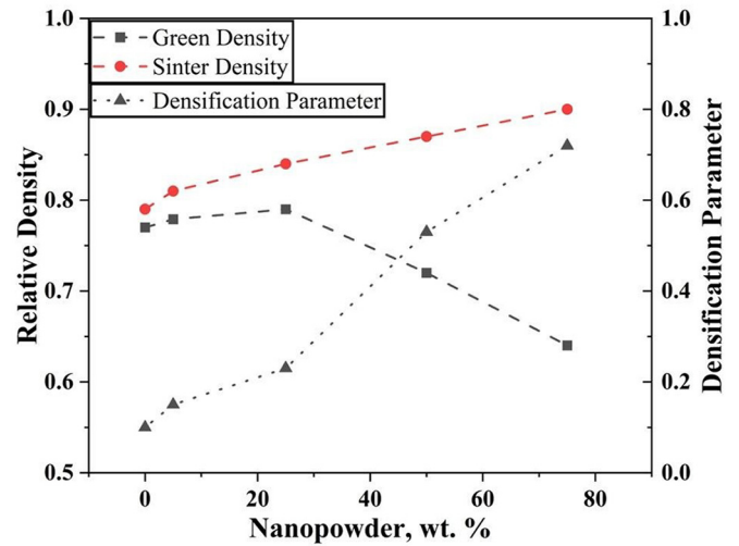
Fig. 4. Relative density and densification parameter of water-atomized iron powder (ASC 300) compacts with varying amounts of nanopowder.
