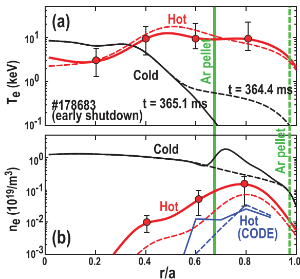
FIG. 9. Reconstructed radial profiles of (a) thermal and non-thermal electron temperature and (b) thermal and non-thermal electron density at two time steps during the early shutdown shot (one at the pellet first impact and one during the pre-TQ). Blue curves show CODE simulations.
