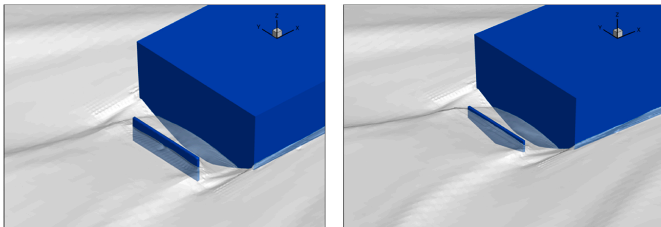
Fig. 15. Application of a rectangular plate (left) and a triangular plate (right) as a TPD.
