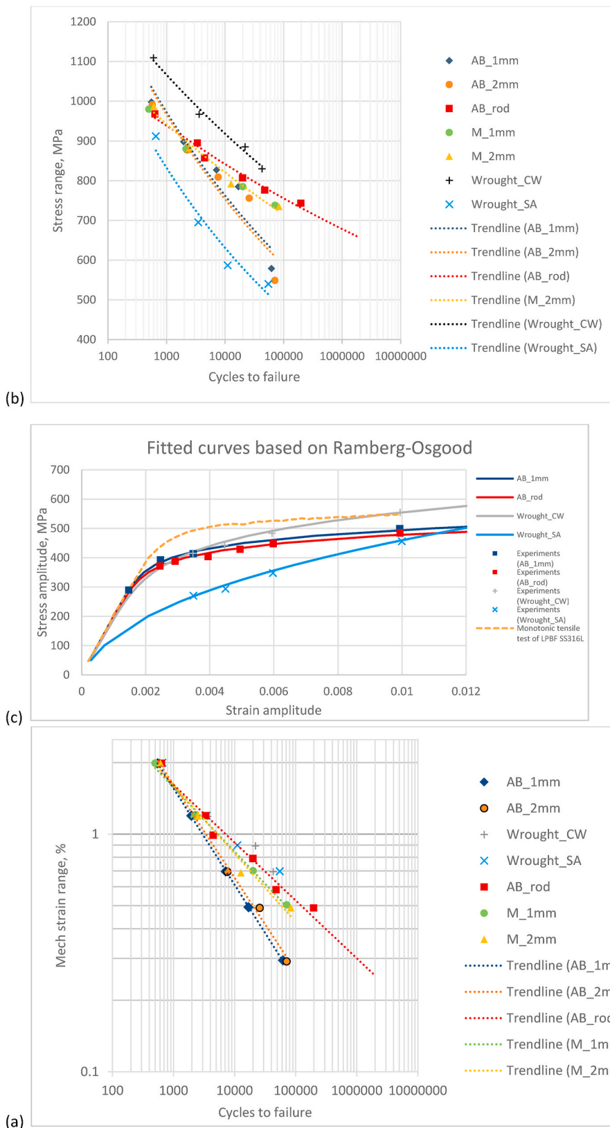
Fig. 7. (a) The applied strain range versus lifetime. Note that it is in log-log plot. (b) The mid-life stress range versus lifetime, where the responding stress range is determined at the mid-life of each applied strain range. Note that the cycle is in log scale. (c) The cyclic stress-strain curves fitted from the Ramberg-Osgood relation, and the experimental results of the applied strain and responding stress are included along the curves. The stress-strain curve of monotonic tensile test is obtained from the first tensile loading cycle of the fatigue test. Note that the trendlines are fitted by using power-law function.
