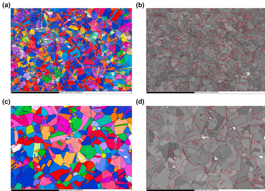
Fig. 6. EBSD grain orientation mapping of the wrought SS 316L, where the loading direction is out-plane. (a) and (b) are from Wrought_CW. (c) and (d) are from Wrought_SA. For (a) and (c), the high angle grain boundaries (>10°) are labelled by the black lines, and the low angle grain boundaries (>2°) are labelled by the grey lines; the colour legend refer to the loading direction. For (b) and (d), both are images from band contrast with the \Sigma 3 {112} incoherent twin boundaries labelled by the red lines. (For interpretation of the references to colour in this figure legend, the reader is referred to the Web version of this article.)
