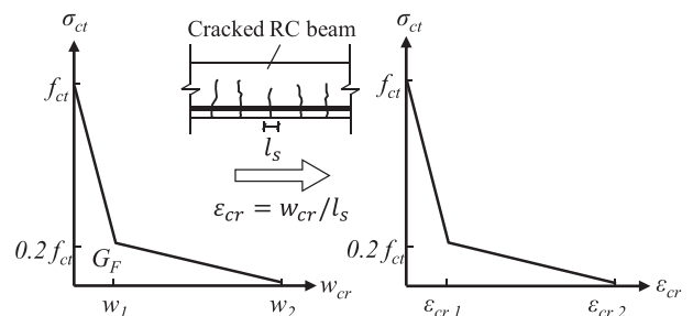
Fig. 3. Bilinear softening curve defined for the post-peak tensile behaviour of concrete converted from stress- w_{cr} relationship according to Model Code 2010 [37].
