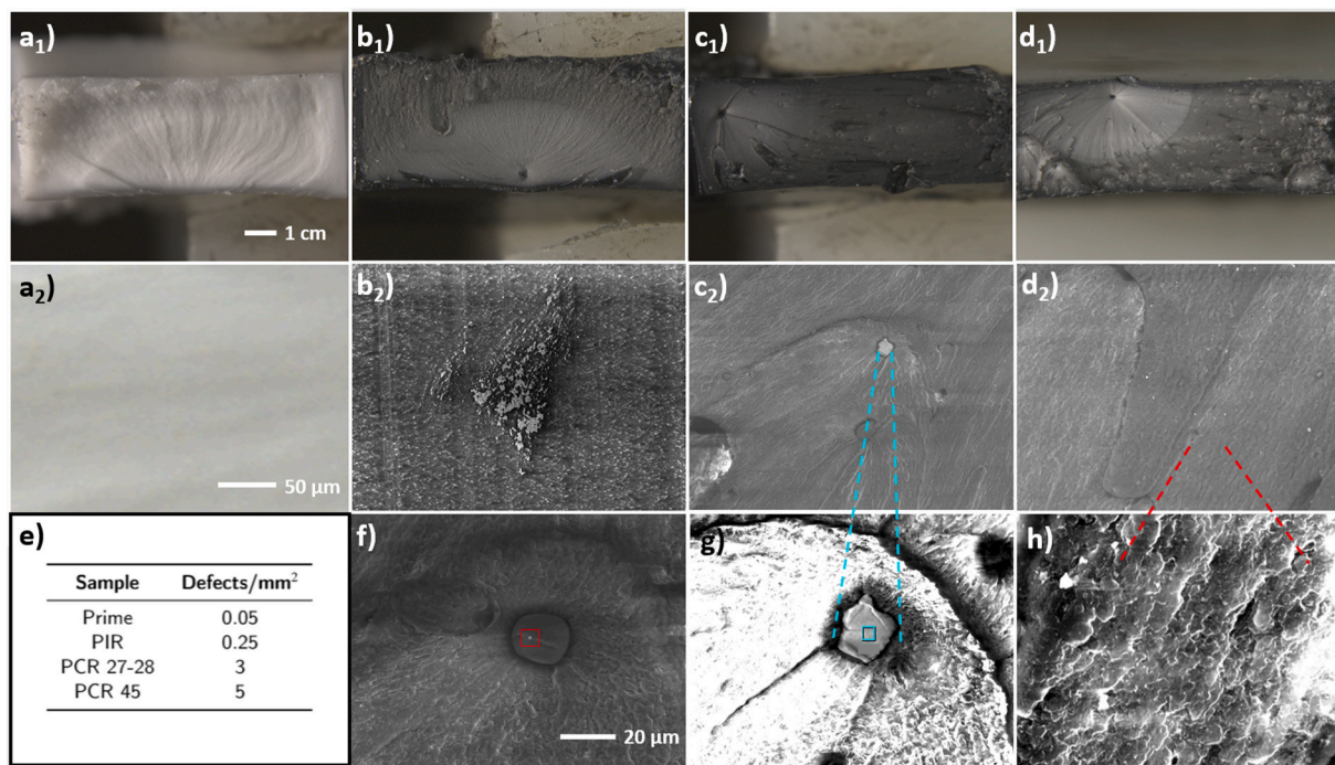
Fig. 4. Series of figures showing tensile fracture surfaces under optical microscopy for Prime (a 1 ), PIR with salt contamination(b 1 ), PCR27-28 (c 1 ) and PCR45 (d 1 ). SEM magnification reveals surface structures in the same sample order for the second row. Total defects/mm 2 are shown in (e). (f) and (g) show magnified SEM images of visible inclusions of ABS agglomeration and an aluminum particle in PCR 27. The red square in (f) is confirmed to be aluminum as well. Close PCR 45 morphology can be seen in (h). Note that inorganic residues were found to be below 2% in TGA analysis. (For interpretation of the references to colour in this figure legend, the reader is referred to the Web version of this article.)
