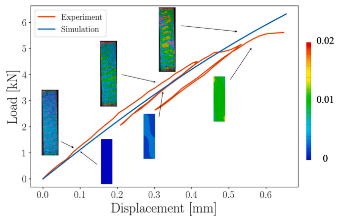
Fig. 12. Load-displacement curve of experimental and predicted results.
