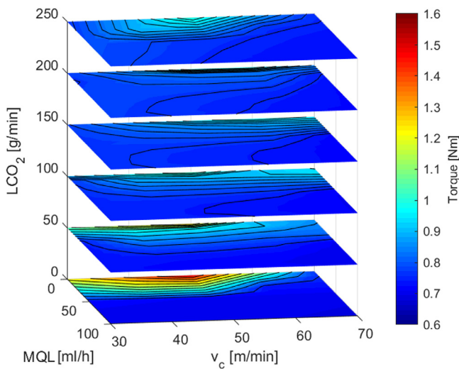
Fig. 4. Torque vs. v_c , q_{LCO_2} and q_{MQL} .
