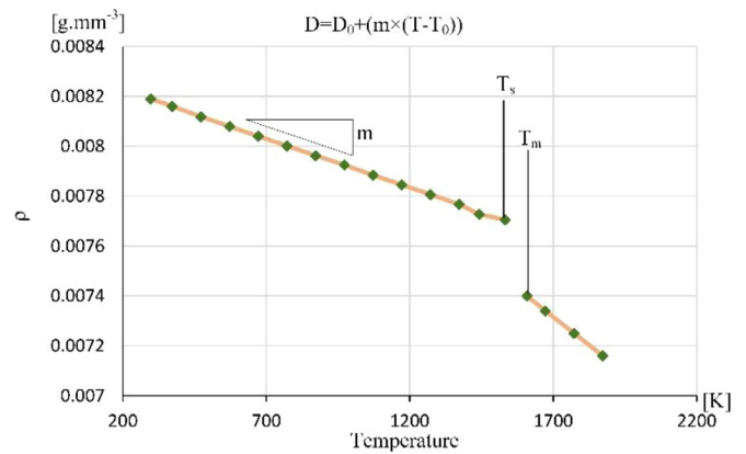
Fig. 2. density versus temperature relationship for Inconel 718 [19].
