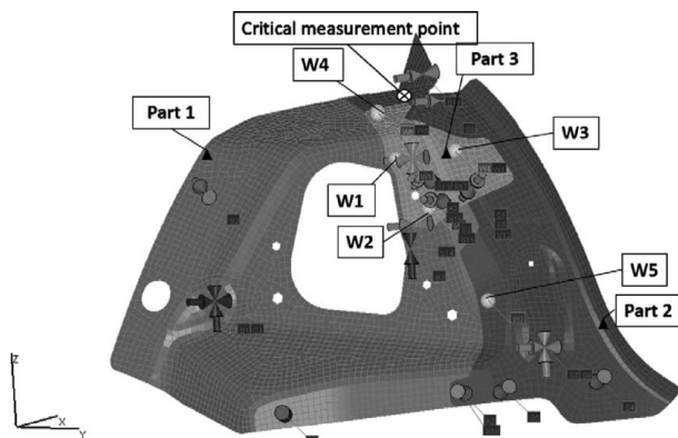
Fig. 6 Assembly B
