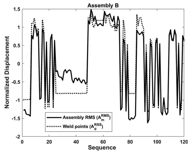
Fig. 9 Assembly B: comparison between A_d^{RSS} and A_m^{RMS}
