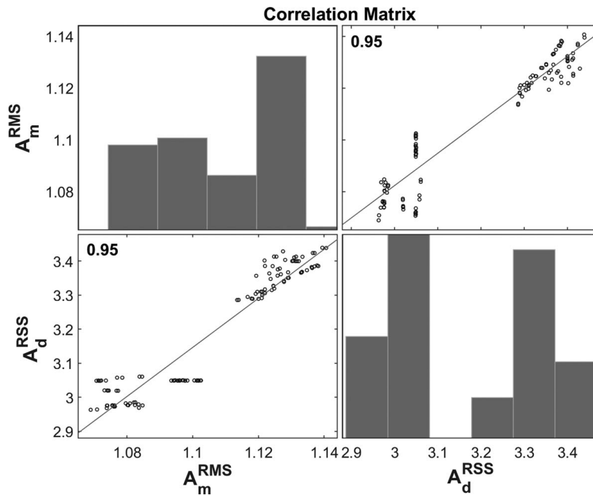
Fig. 10 Assembly B: correlation between A_d^{RSS} and A_m^{RMS}
