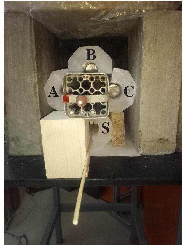
Fig. 2: A picture of the measurement setup.
