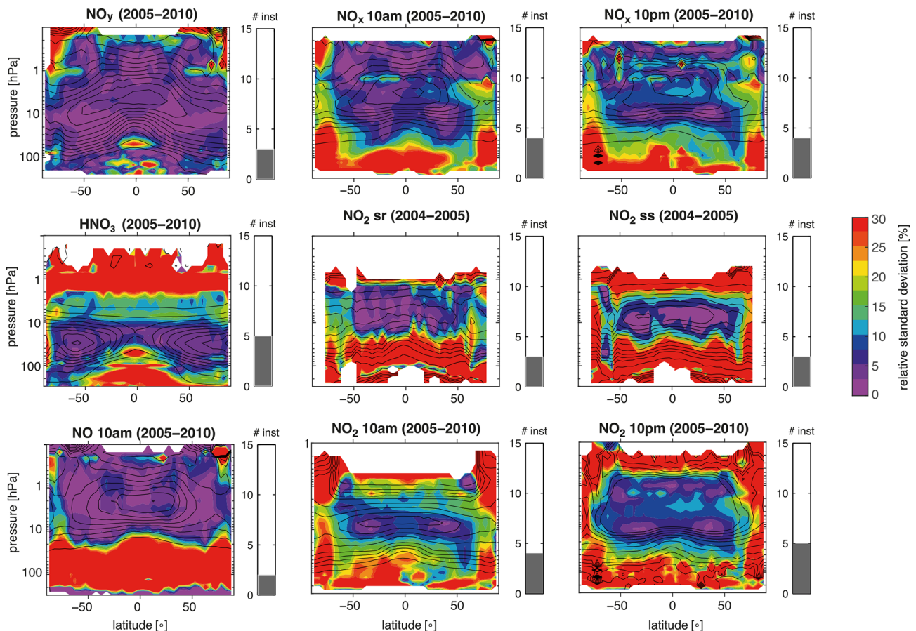
Figure 16. Same as Fig. 14 but for nitrogen-containing species. The assessment of the uncertainty in the annual mean state of \text{NO} , \text{NO}_x , and \text{NO}_2 is based on gridded datasets corresponding to 10:00 and 22:00 LT, and for the latter also on datasets corresponding to local sunrise (sr) and local sunset (ss). Note that some of the included datasets have been derived by scaling the individual measurements with a chemical box model to 10:00 and 22:00 local solar time (LST). See SPARC (2017) for more detailed information. Reactive nitrogen ( \text{NO}_x ) is here defined as \text{NO} + \text{NO}_2 . The odd nitrogen family ( \text{NO}_y ) is defined as \text{NO}_x + \text{HNO}_3 + 2 \times \text{N}_2\text{O}_5 + \text{ClONO}_2 + \text{HNO}_4 . For \text{N}_2\text{O}_5 , \text{ClONO}_2 , and \text{HNO}_4 , an assessment of the uncertainty in the annual mean field cannot be provided since no data products at the same local solar time are available.
