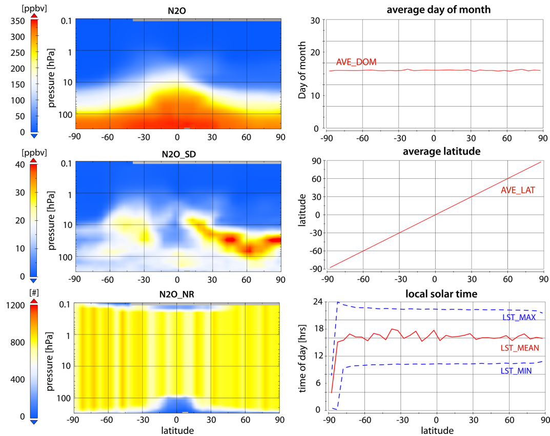
Figure 5. Variables in a typical data file that follows SPARC Data Initiative standards are \text{N}_2\text{O} volume mixing ratio, \text{N}_2\text{O} standard deviation ( \text{N}_2\text{O\_SD} ), \text{N}_2\text{O} number, average day of month, average latitude, and minimum, mean, and maximum local solar time (LST_MIN, LST_MAX, and LST_MEAN). This example shows April data from the 2008 MIPAS zonal monthly mean file.
