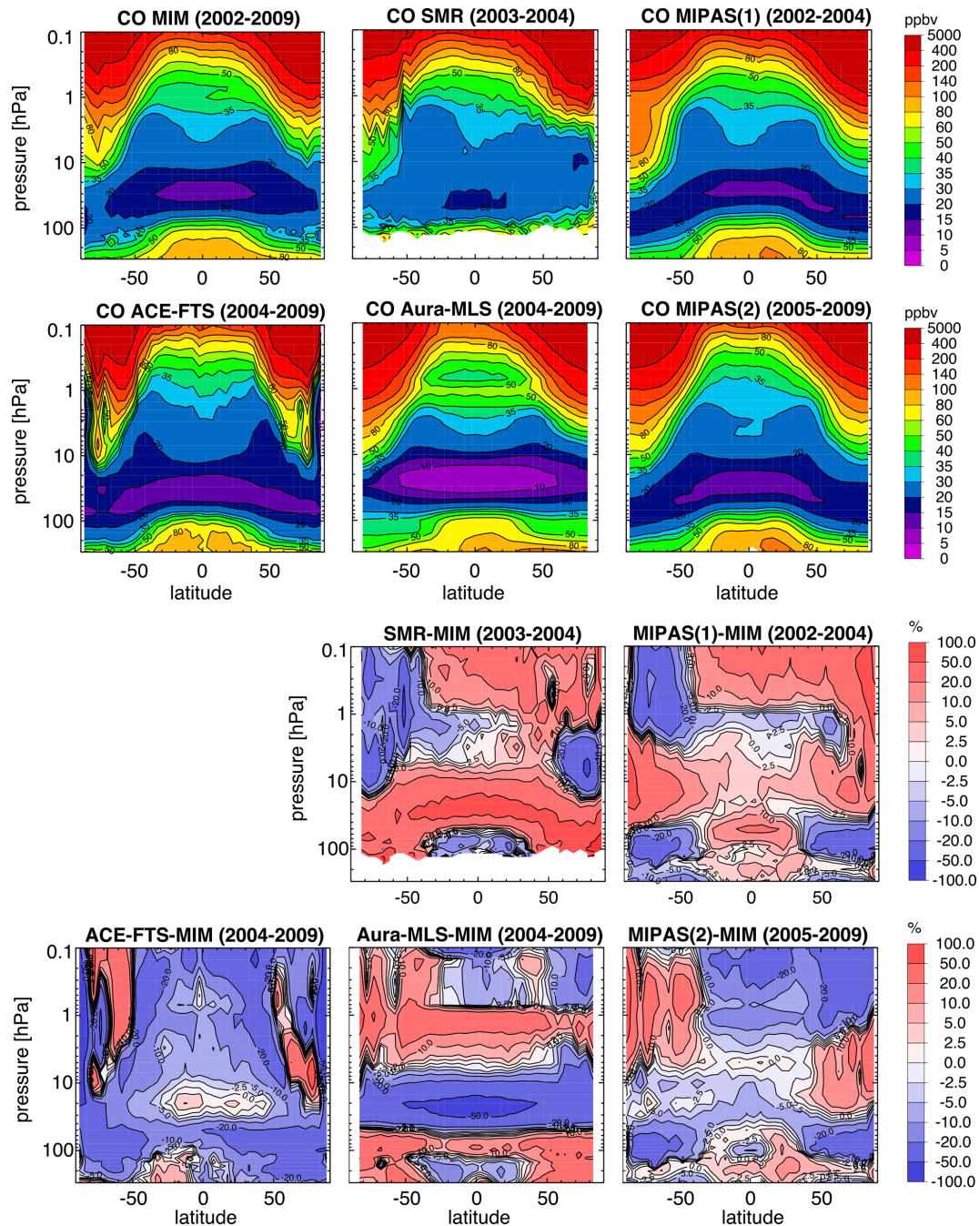
Figure 10. Annual zonal mean CO cross sections are shown for the MIM, SMR, MIPAS(1), ACE-FTS, MIPAS(2), and Aura-MLS averaged over 2002–2009 (upper half). Also shown are the relative differences between the individual instruments and the MIM (lower half). Note that SMR and MIPAS(1) are excluded from the calculation of the MIM.
