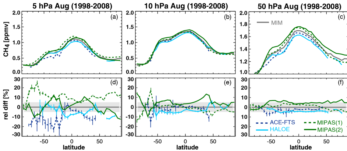
Figure 8. Meridional profiles of zonal monthly mean CH 4 at 5, 10, and 50 hPa and averaged over 1998–2008 are shown for the different instruments and the MIM (a, b, c). Differences between the individual instruments and the MIM are shown in the lower panels (d, e, f). The grey shading indicates where the relative differences are smaller than \pm 5\% (thus where the datasets show very good to excellent agreement). Error bars indicate the uncertainty in the relative differences based on the SEM of each instrument.
