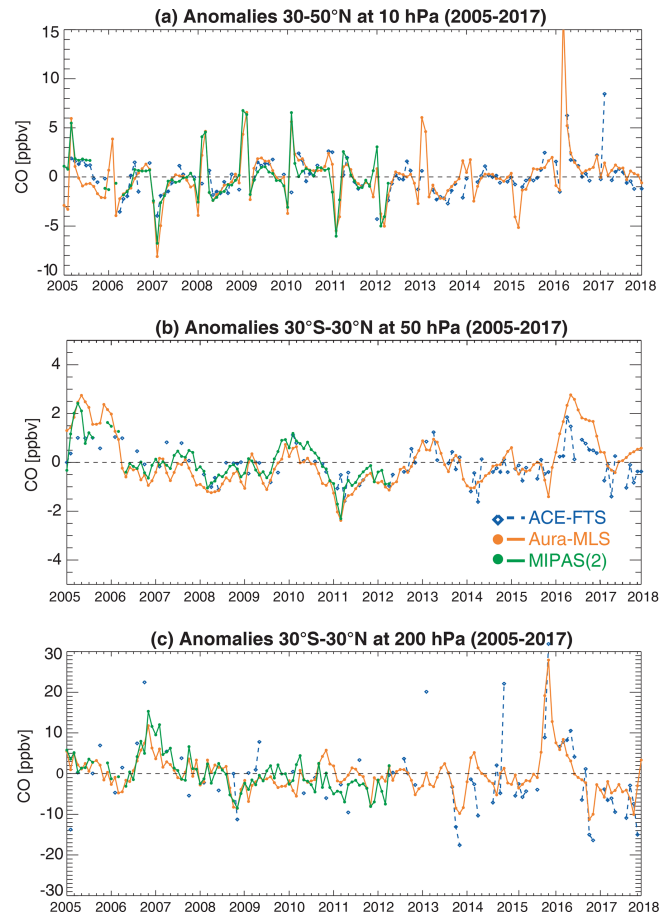
Figure 11. Deseasonalized CO anomalies from ACE-FTS, MIPAS(2), and Aura-MLS are shown for 30°–50° N at 10 hPa (a), and 50 hPa (b) and 200 hPa (c) for 30° S–30° N and the time period 2005–2017.
