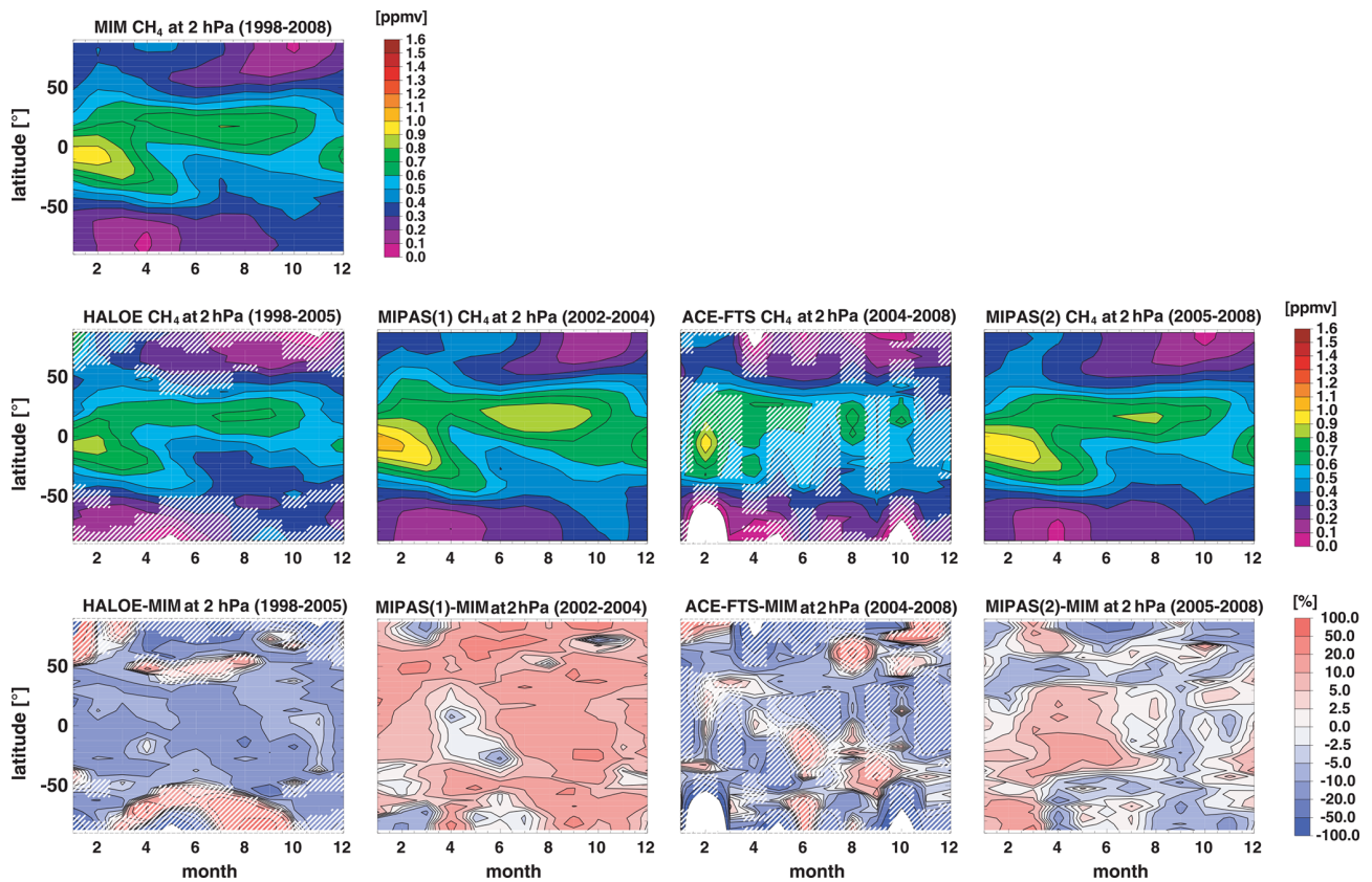
Figure 9. Latitude–time evolution of zonal monthly mean CH 4 at 2 hPa and averaged over 1998–2008. Shown are absolute values for the MIM (top panel) and the different instruments (middle row), and for the relative differences with respect to the MIM (lower row). Note that HALOE and ACE-FTS show linearly interpolated fields, with hatched regions indicating where no measurements are available.
