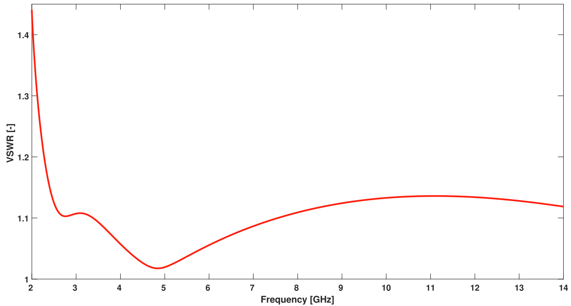
Fig. 9. Voltage Standing Wave Ratio (VSWR) of the Archimedean spiral antenna as a function of frequency, over the frequency range 2–14 GHz. Except of the first 500 MHz where there is a 30% increase in VSWR, the spectrum is stable within less than 10% variability.
