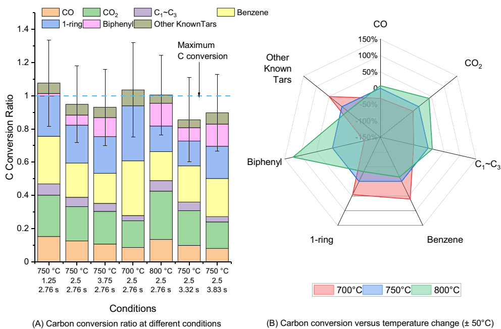
Fig. 6. Carbon balance of PET steam gasification experiments.
