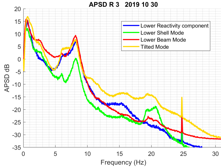
Figure 4.3: APSDs of the beam mode, shell mode, reactivity component and the tilting mode for the lower detectors, extracted from Measurement 1
