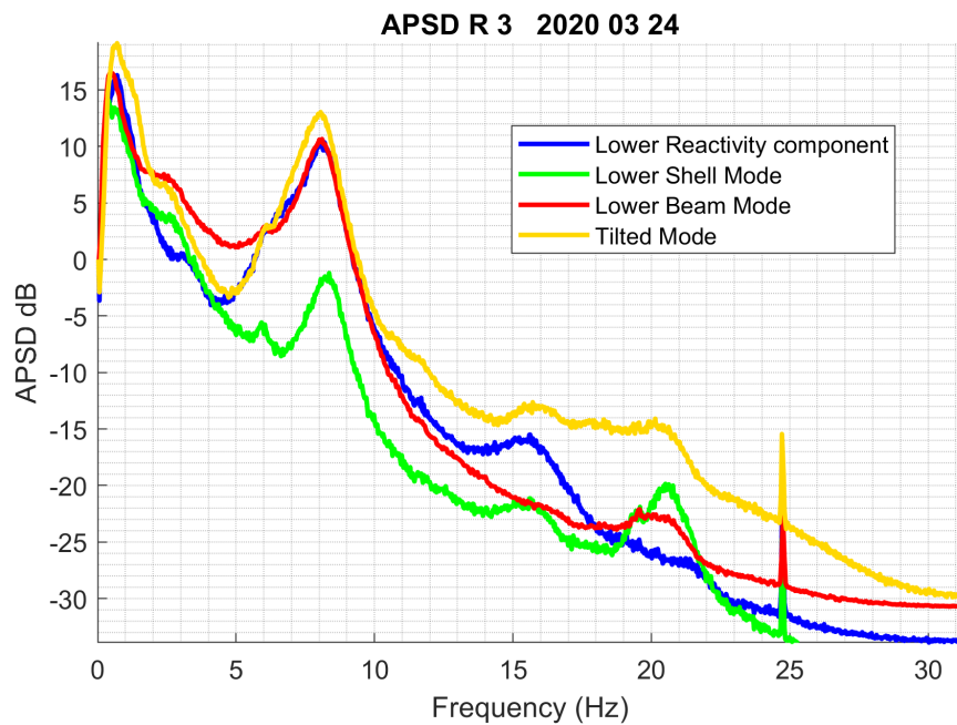
Figure 4.15: APSDs of the beam mode, shell mode, reactivity component and the tilting mode for the lower detectors, extracted from Measurement 3.
