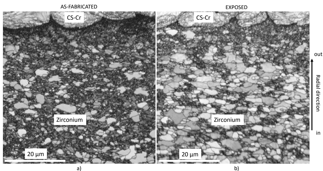
Figure 5-3: EBSD maps over as-fabricated (a) and autoclave exposed (b) CS-Cr coated Optimized ZIRLO cladding cross-sections (Map size 50x50 \mu\text{m} ).
