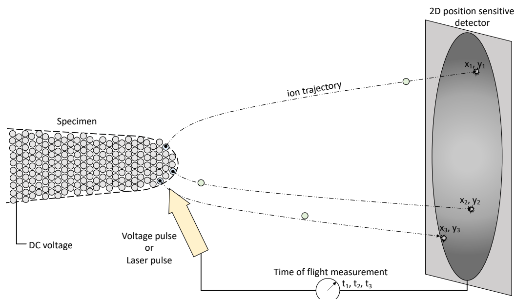
Figure 4-7: Schematic of APT working principle.
