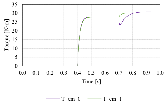
Fig. 7 Waveforms of electromagnetic torque.
