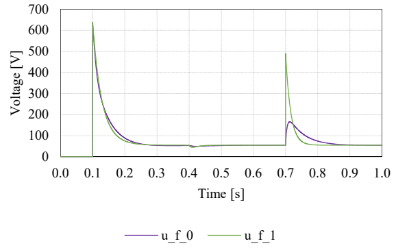
Fig. 6 Waveforms of field voltage.
