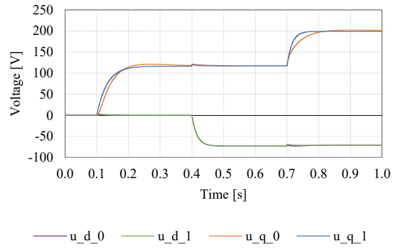
Fig. 5 Waveforms of d- and q-axis voltages.
