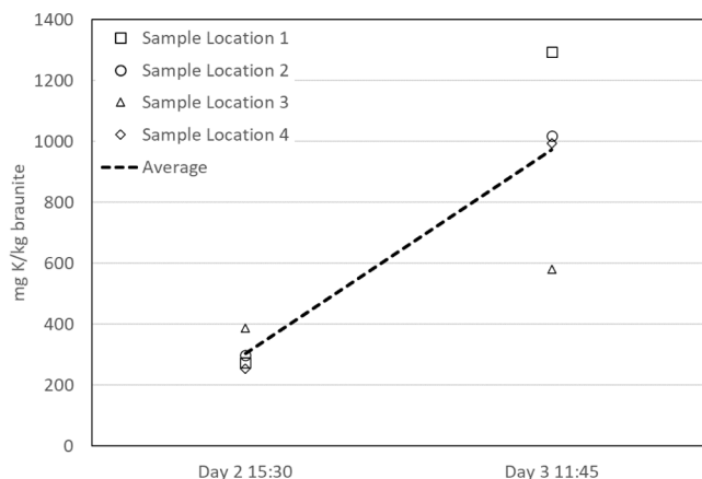
Fig. 10. Potassium content of braunite samples.
