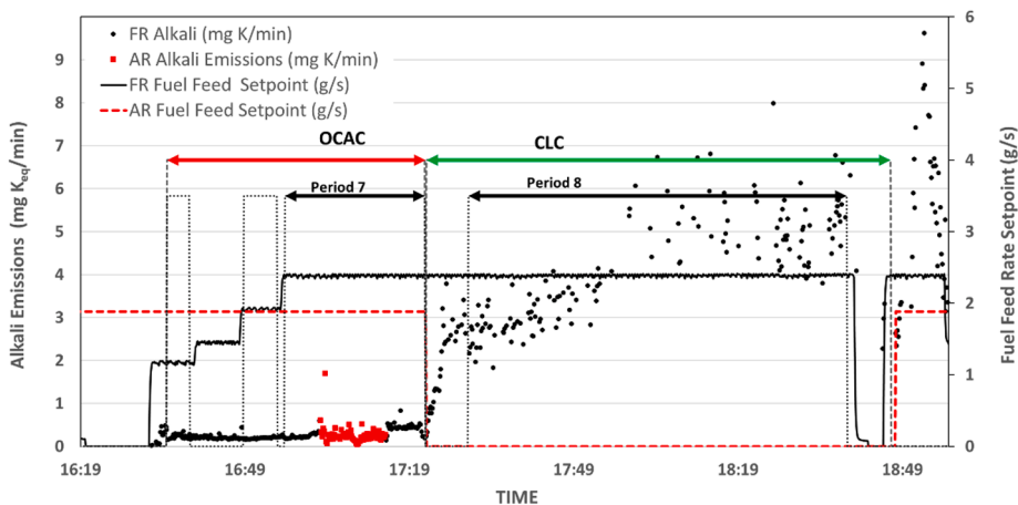
Fig. 4. Alkali emissions for Test 3 (ilmenite & wood char).
