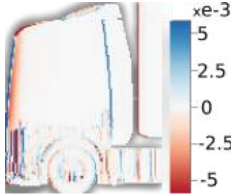
Figure 4.12: Trailing truck difference in drag between 20m and 2.5m
