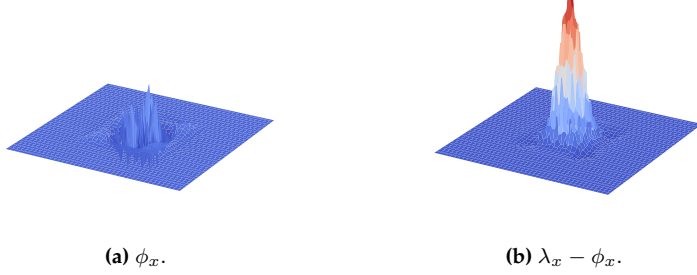
Figure 2: The basis correction \phi_x (left) and corresponding modified basis function \lambda_x - \phi_x (right) for a coarse node x \in \mathcal{N} positioned at (0.375, 0.500) in the unit square.
