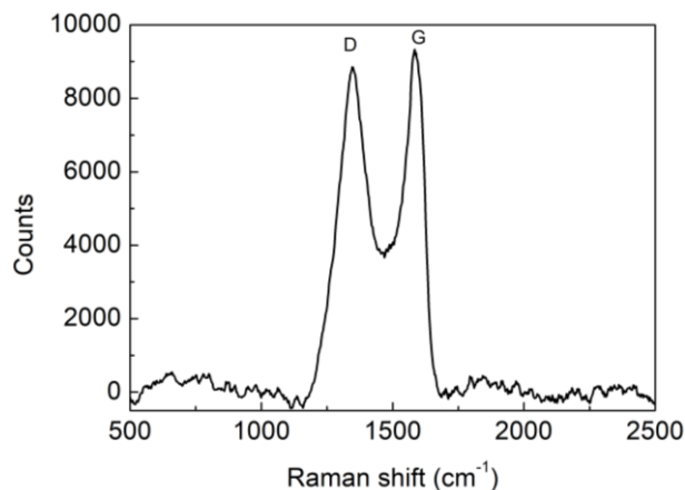
Figure 25: Raman spectrum of GO on unsintered Cu particle.
