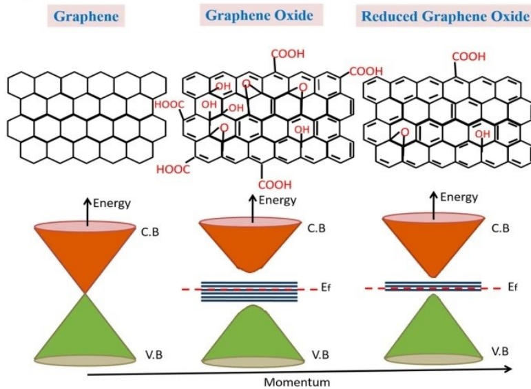
Figure 4: Electronic band structure of graphene, GO and reduced GO. Adapted from Sehrawat et al. [23] under the Creative Commons license .
