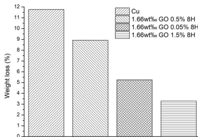
Figure 43: Weight loss in CuGO after etching in 10% acetic acid for 7 days. The CuGO was synthesized by functionalizing Cu with APTES for 8 hours.
