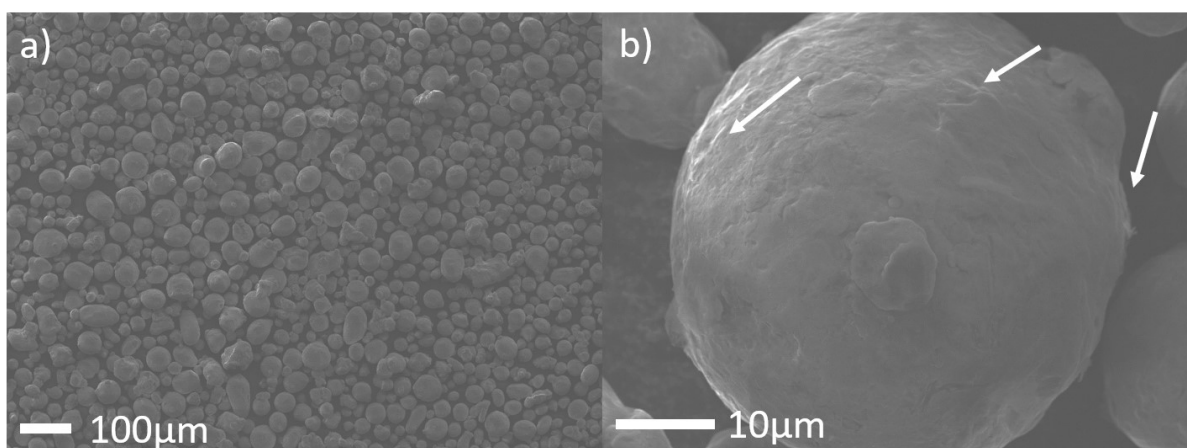
Fig. 1: SEM images of p-thick-GO@Cu powder (0.625wt% GO ratio and 2.5vol% APTES) under a) low and b) relatively high magnification. No clustering was observed, and graphene was uniformly coated on Cu particles.
