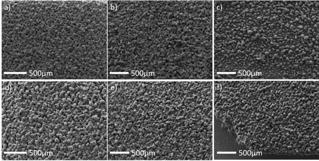
Fig. 11: SEM images of Cu powder sintered with SLS. The Cu powders in the top row were sintered with a) 160 W, b) 140 W and c) 120 W at 700 mm/s. The other samples were sintered with 160 W powder and d) 400 mm/s, e) 500 mm/s and f) 600 mm/s.
