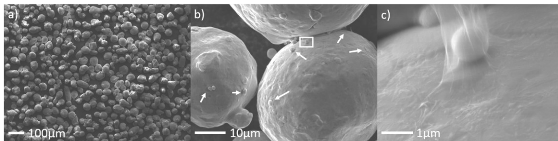
Figure 2: GO@Cu powder synthesized with 0.625wt% GO and 0.2% APTES for 30 minutes.
