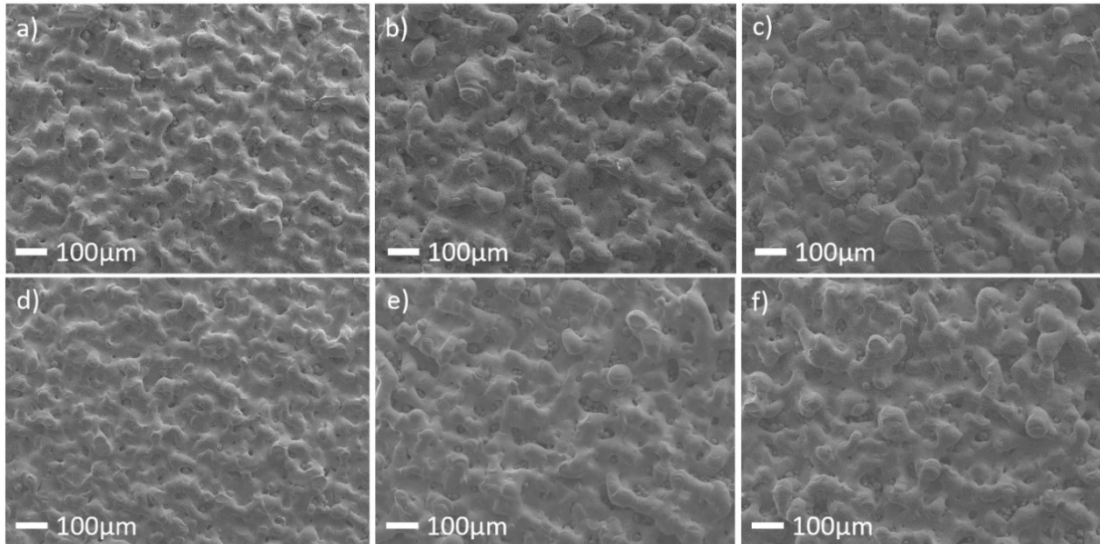
Fig. 12: SEM images of the GO@Cu powder sintered with SLS. The GO@Cu powders in the top row were sintered with 700 mm/s scan speed and a) 160 W, b) 140 W and c) 120 W laser power. The lower row was sintered at 160 W and d) 400 mm/s, e) 500 mm/s and f) 600 mm/s scan speed
