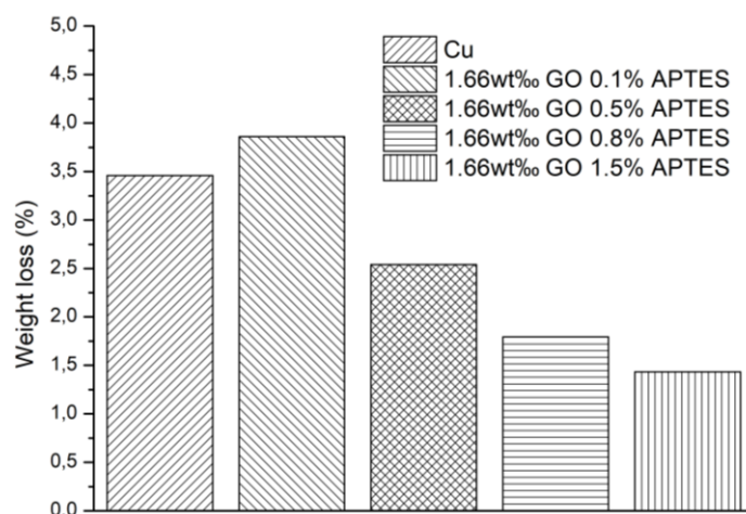
Figure 41: Weight loss in CuGO after etching in 10% acetic acid for 2,5 hours.
